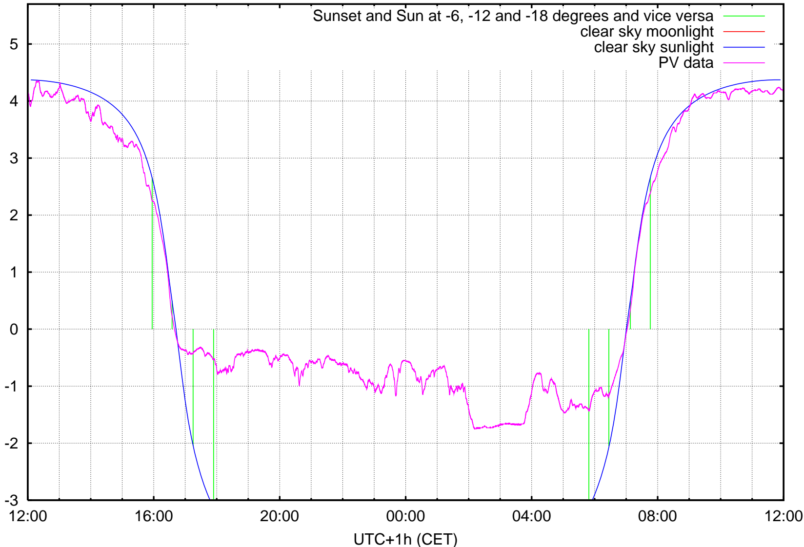
log10 ( illuminance / 1 lx ) Kravi hora, Brno, ending at Thursday 2006-12-21 noon
