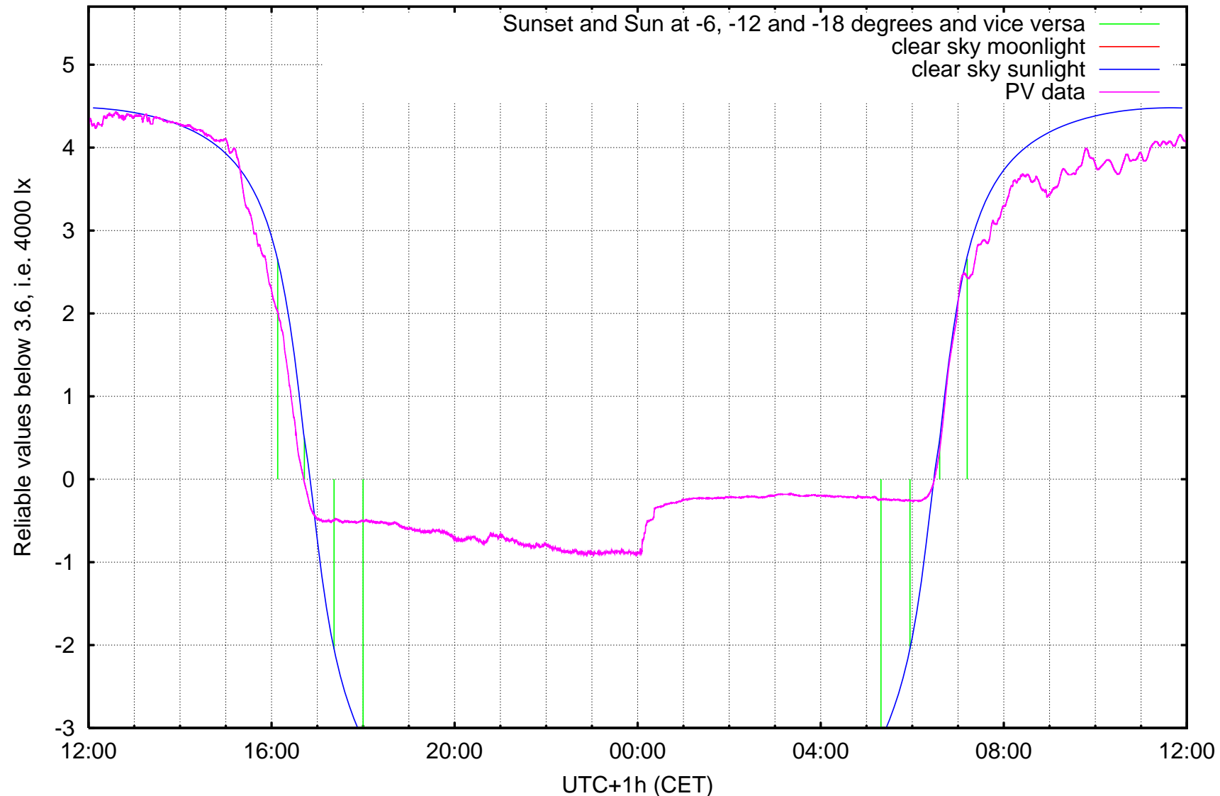
log10 ( illuminance / 1 lx ) Kravi hora, Brno, ending at Monday 2006-11-20 noon
