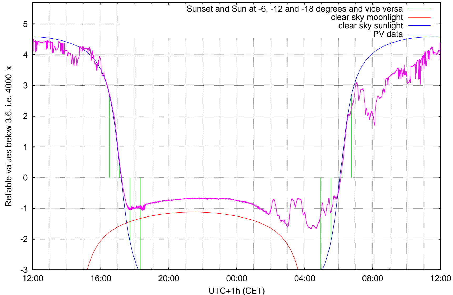
log10 ( illuminance / 1 lx ) Kravi hora, Brno, ending at Friday 2006-11-03 noon
