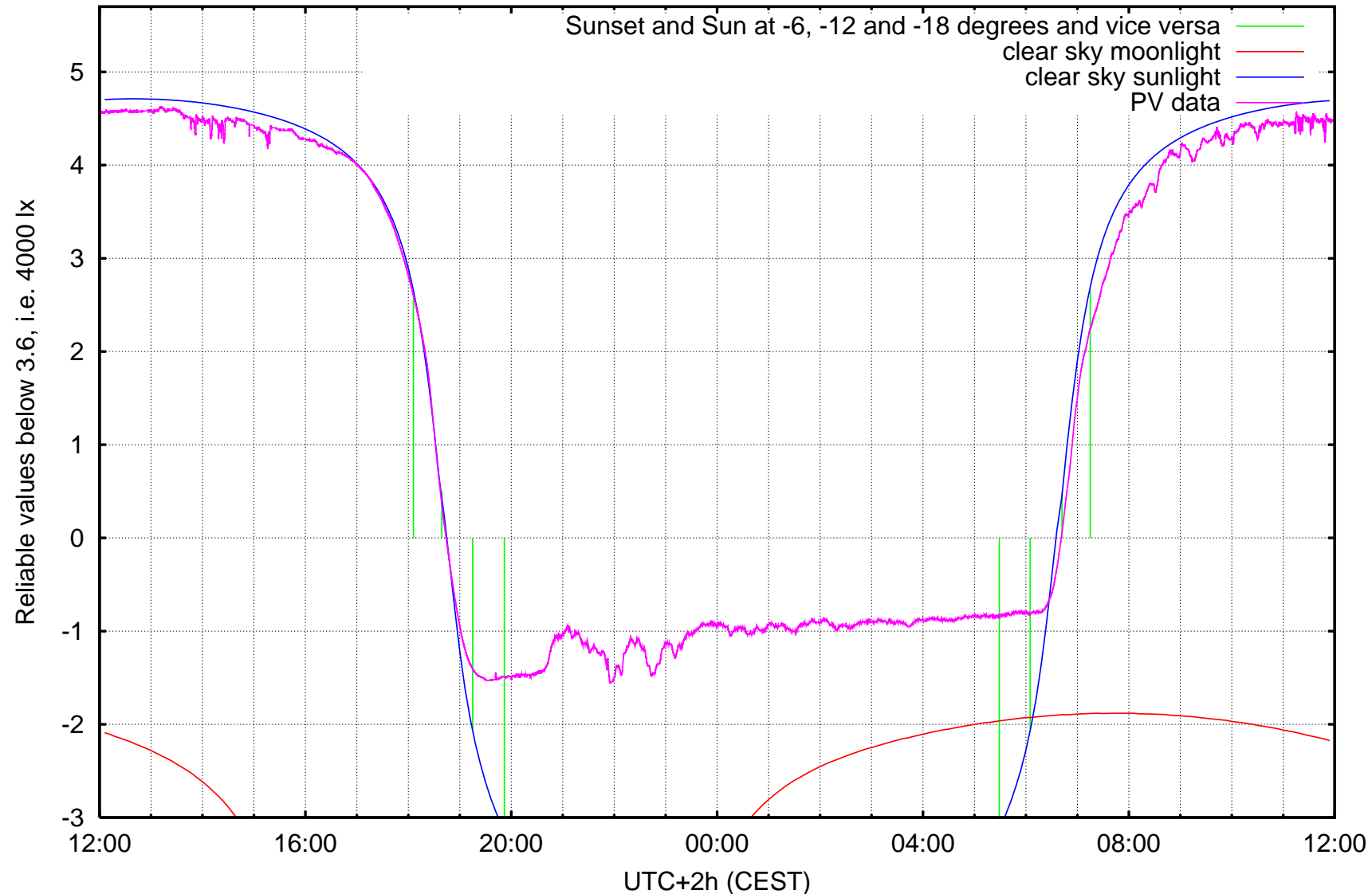
log10 ( illuminance / 1 lx ) Kravi hora, Brno, ending at Sunday 2006-10-15 noon
