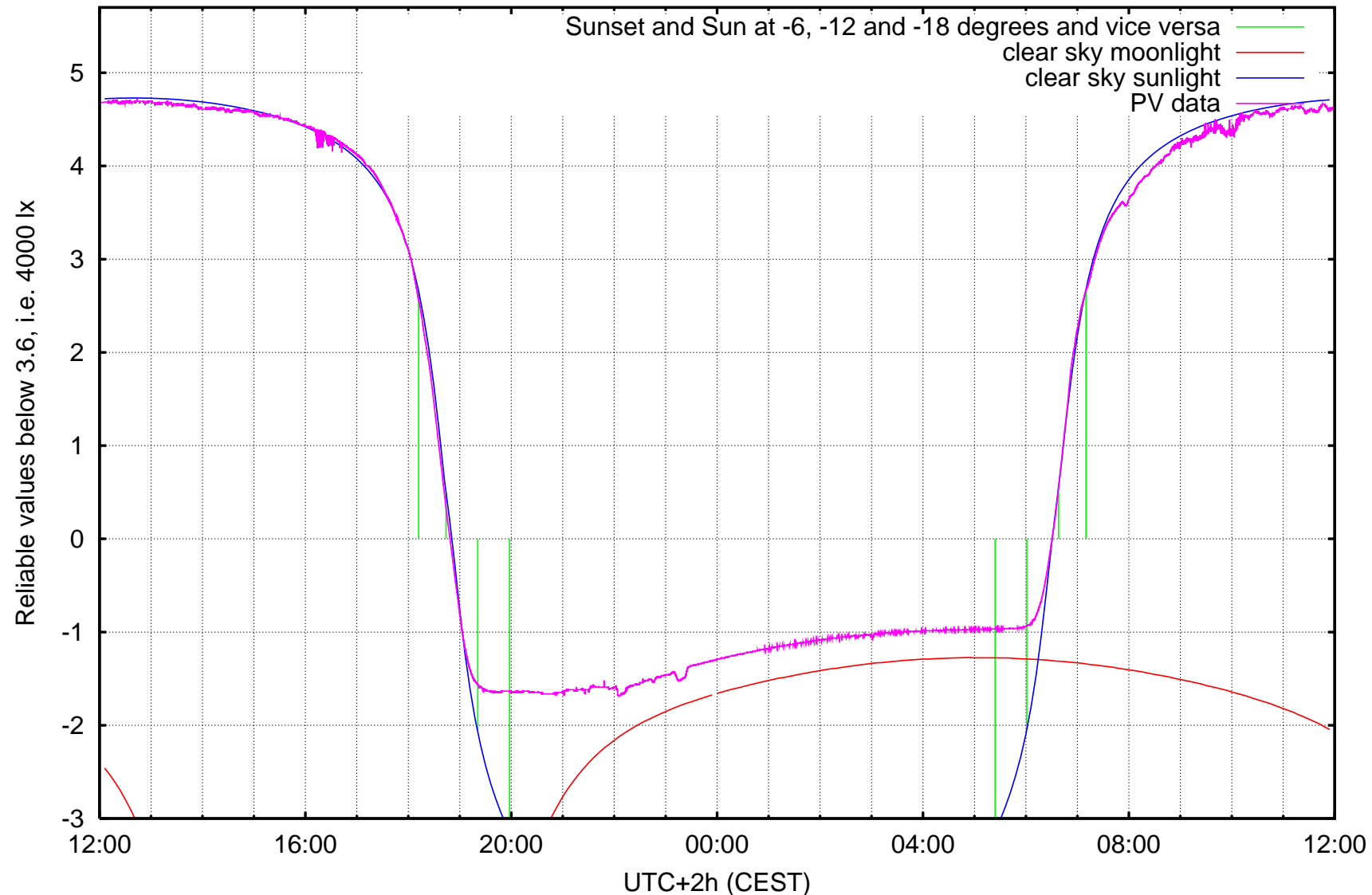
log10 ( illuminance / 1 lx ) Kravi hora, Brno, ending at Thursday 2006-10-12 noon
