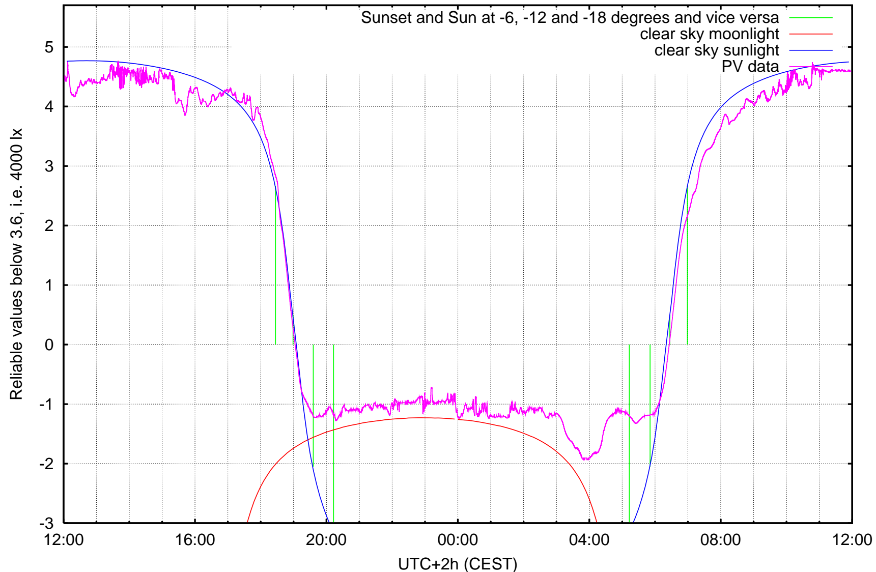
log10 ( illuminance / 1 lx ) Kravi hora, Brno, ending at Thursday 2006-10-05 noon
