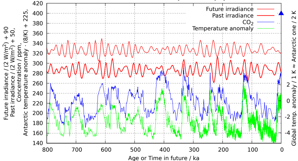
Irradiance of atmosphere, CO 2 , temperature anomaly: past 800 thousand years and irradiance in next 800 thousand years, mid July at 65° latitude
