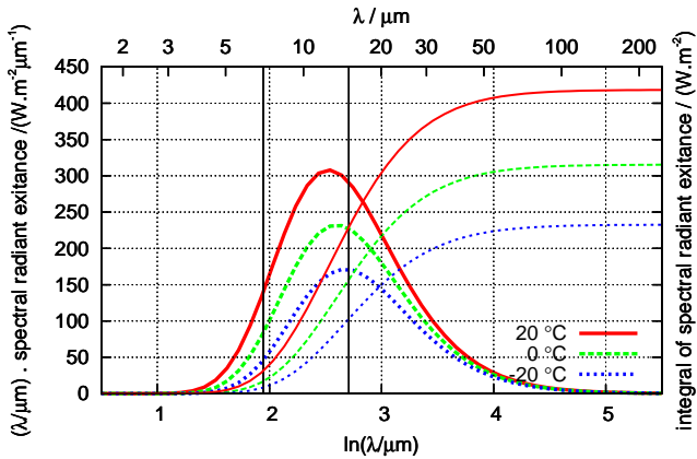
Blackbody radiation, log scale \lambda - Planck functions and their integrals (the LWIR band from 7 \mu\text{m} to 15 \mu\text{m} is marked)
