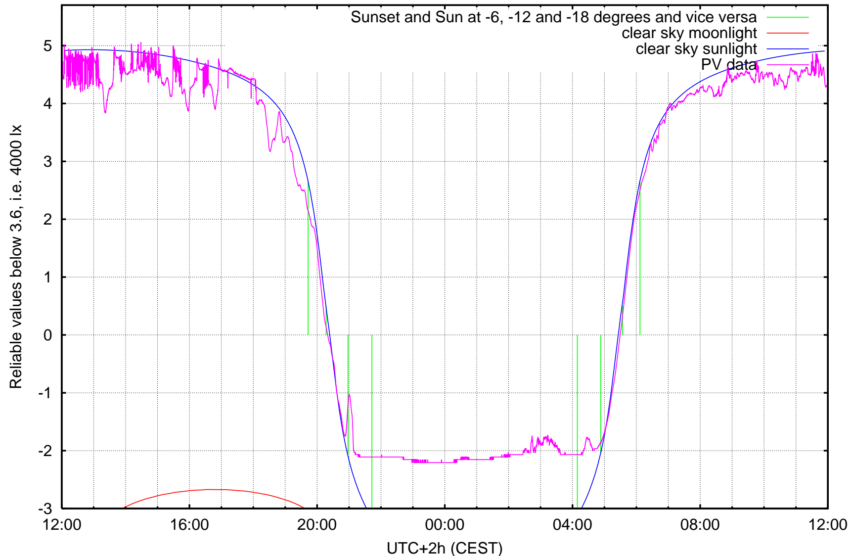
log10 ( illuminance / 1 lx ) Kravi hora, Brno, ending at Wednesday 2006-08-30 noon
