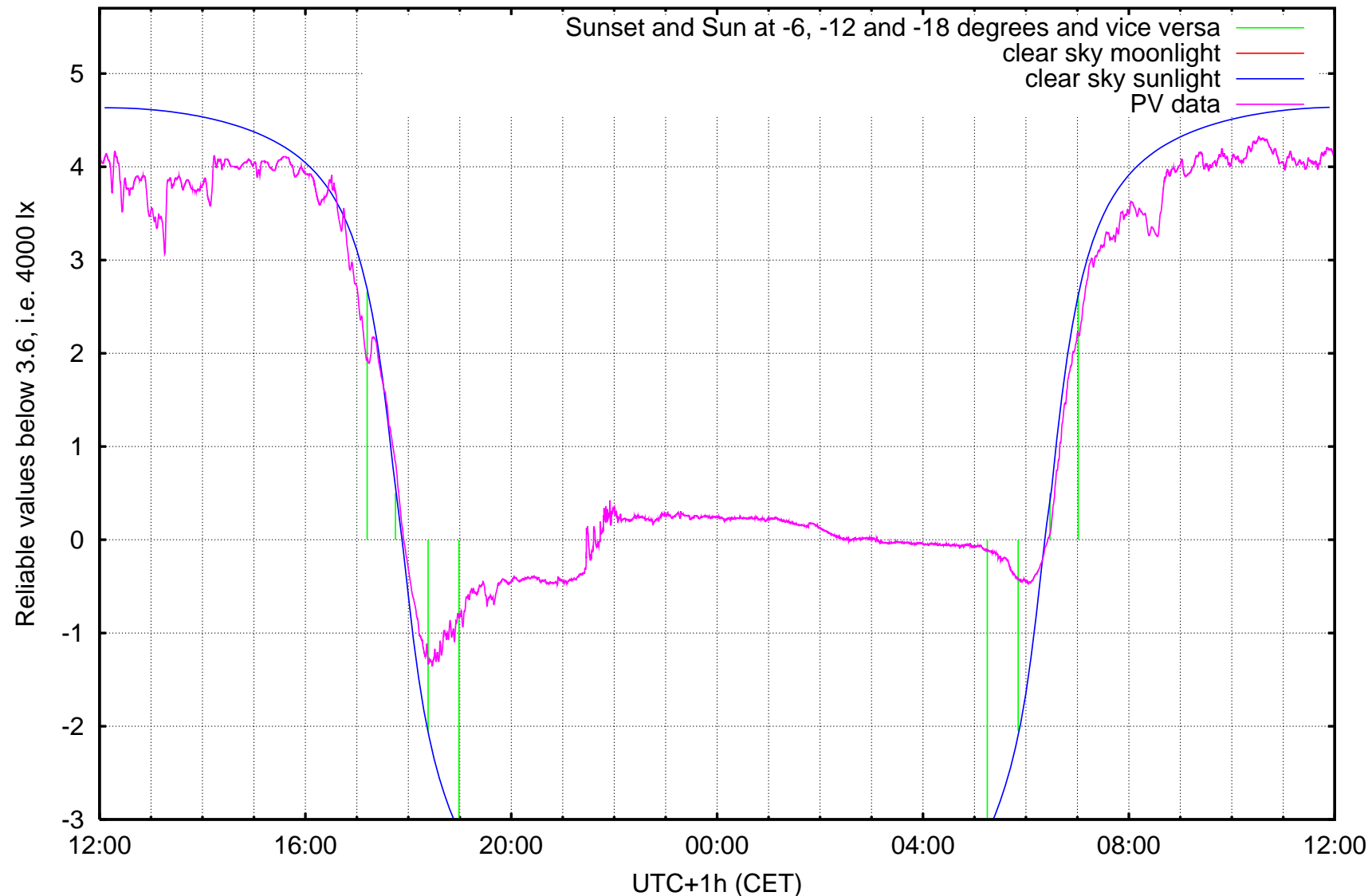
log10 ( illuminance / 1 lx ) Kravi hora, Brno, ending at Friday 2007-02-16 noon
