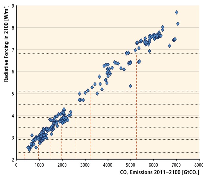
Figure A.II.8. Regression of radiative forcing against 2011-2100 cumulative CO 2 emissions. Scenarios of full forcing models GCAM, MERGE, MESSAGE, REMIND and IMAGE were used for this analysis. Regression was done separately for each model, and resulting budget ranges averaged across models.
