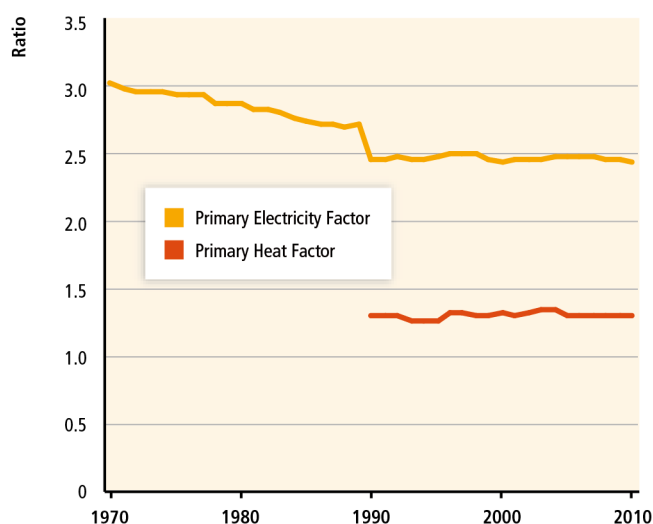
Figure A.II.3. Historical primary electricity and heat factors. Data source: (IEA, 2012b)
