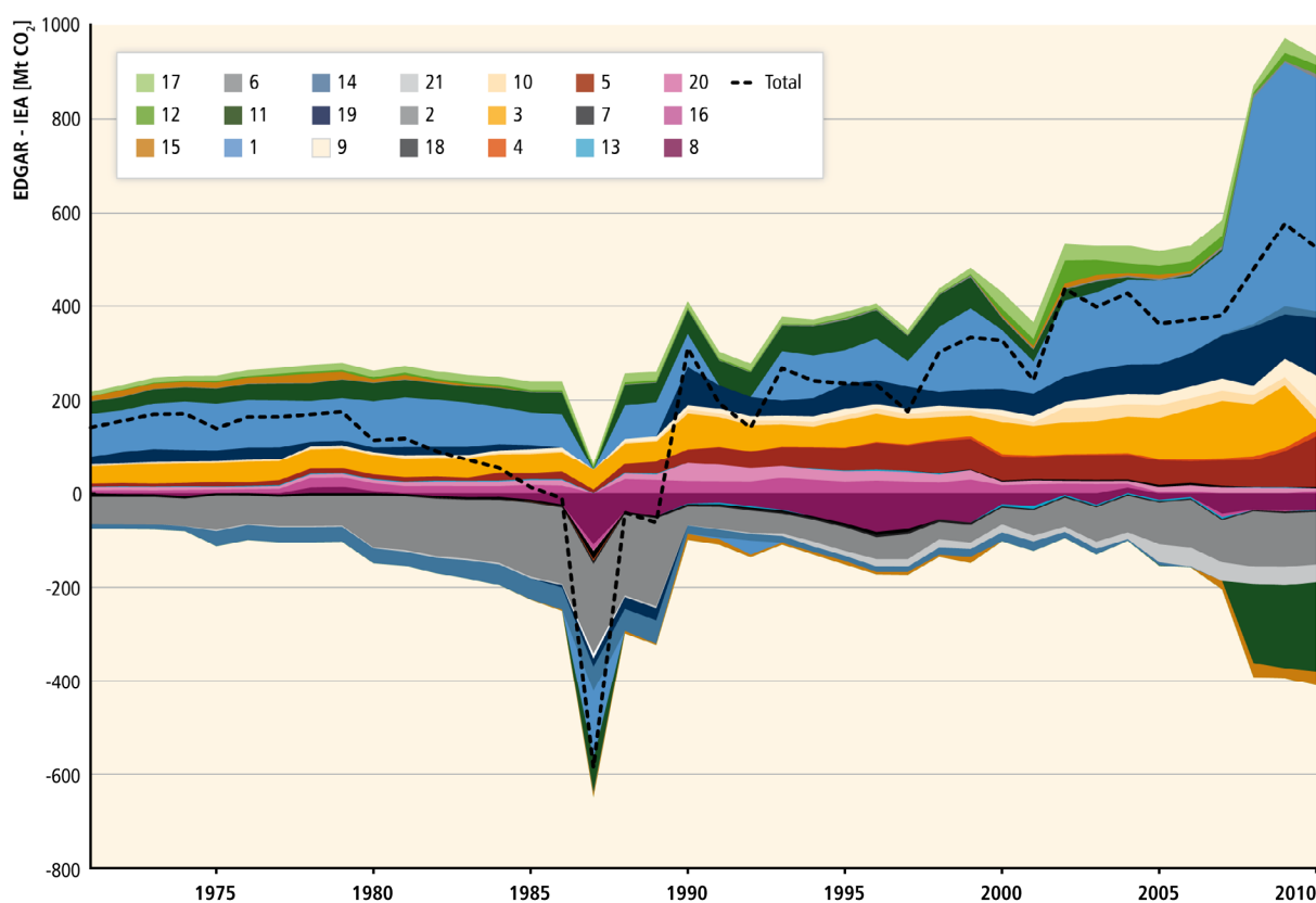
Figure A.II.7. Difference of CO 2 emissions between analogous IEA (2012c) and EDGAR (JRC/PBL, 2012) categories as detailed in Table A.II.11. (Numbers in key refer to Table A.II.11 Comparison Groups).
