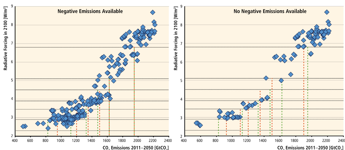
Figure A.II.9. Regression of radiative forcing against 2011–2050 CO 2 emissions. Red lines show mean results of fit and depend on whether (left panel) or not (right panel) negative emissions are available. Green lines show harmonized bins between both categories for the mapping in Table A.II.19.
