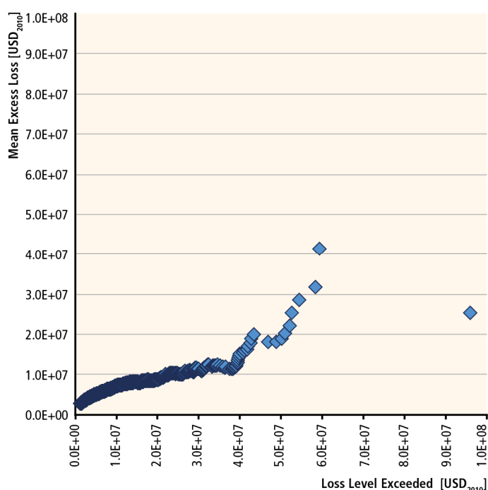
Figure A.II.6. Mean excess curve of US crop insurance indemnities paid from the US Department of Agriculture's Risk Management Agency, aggregated by county and year for the years 1980 to 2008 in USD 2010 .
