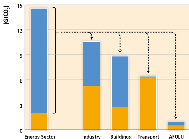
Figure A.II.2. Energy sector electricity and heat CO 2 emissions calculated for the end-use sectors in 2010. Data source: (IEA, 2012b; c)
