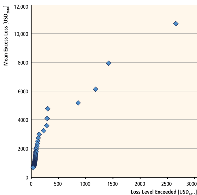
Figure A.II.5. Mean excess curve for US flood insurance claims from the National Flood Insurance Program per dollar income per county per year for the years 1980 to 2008 in USD 2010 . Considering dollar claims per dollar income in each county corrects for increasing exposure.
