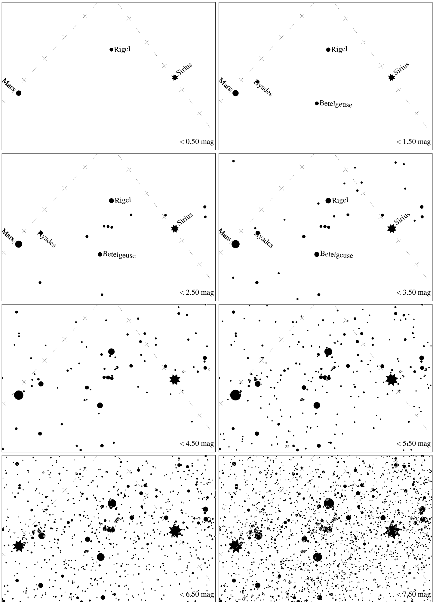
Maps for Globe at Night at latitude -20^\circ , 2023-01-09, 21 h local time (Sun at -28^\circ ), transparent air. Lines from N(E,S,W) to zenith shown (crosses each 10^\circ ). Orion 's belt is 49^\circ to the right from N, at 63^\circ height. Star clusters M 41 and M35 marked when appropriate. Map vertical size is 50^\circ . Jan Hollan maps, CzechGlobe
