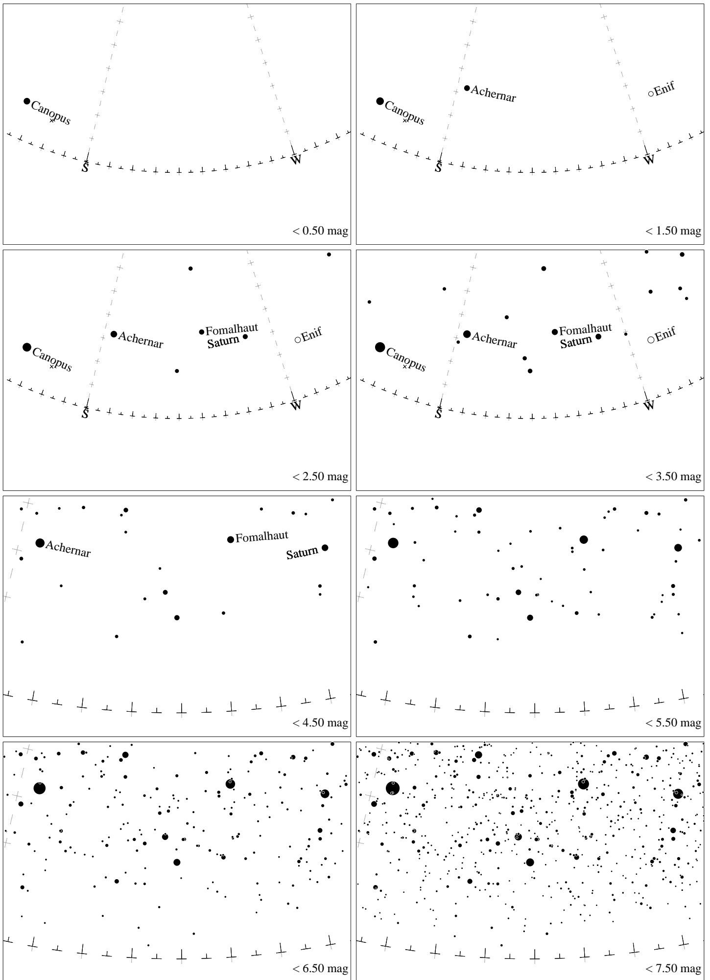
Maps for Globe at Night latitude 0°, 2023-12-08, 21 h local time (Sun at -42^\circ ), transparent air. Lines from N(E,S,W) to zenith shown (crosses each 10^\circ ). Centered on Alnair ( \alpha Gruis), which is 39^\circ to the right from S, at 20^\circ height. Detailed maps 50^\circ vertically, the first four maps 100^\circ . Jan Hollan, CzechGlobe
