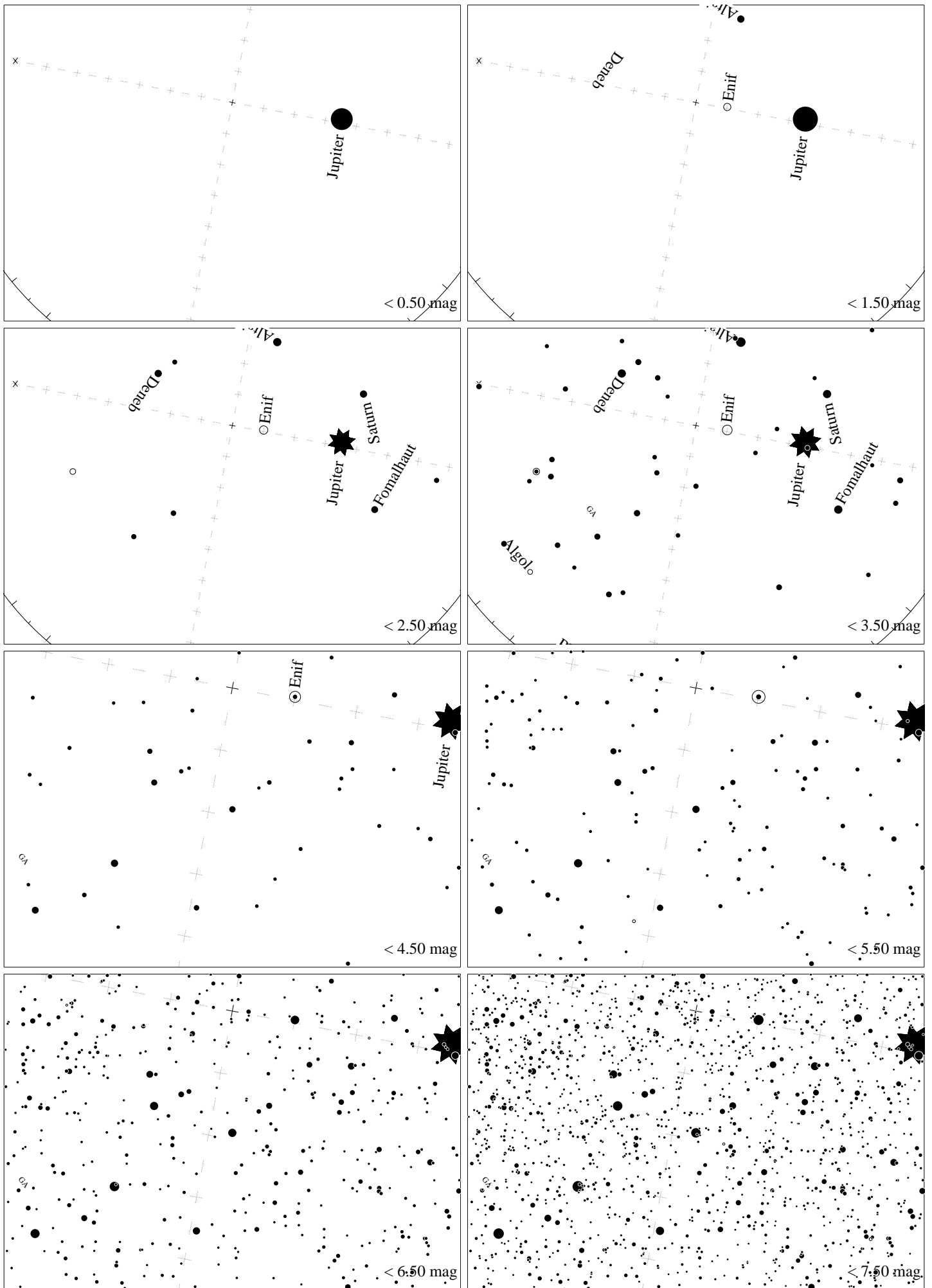
Maps for Globe at Night latitude 20°, 2021-10-02, 21 h local time (Sun at -46^\circ ), transparent air. Lines from N(E,S,W) to zenith shown (crosses each 10°). The map is centered on Markab ( \alpha Pegasi), which is 79^\circ to the left from S, at 71^\circ height. Detailed maps 50^\circ vertically, the first four maps 100^\circ . Jan Hollan, CzechGlobe
