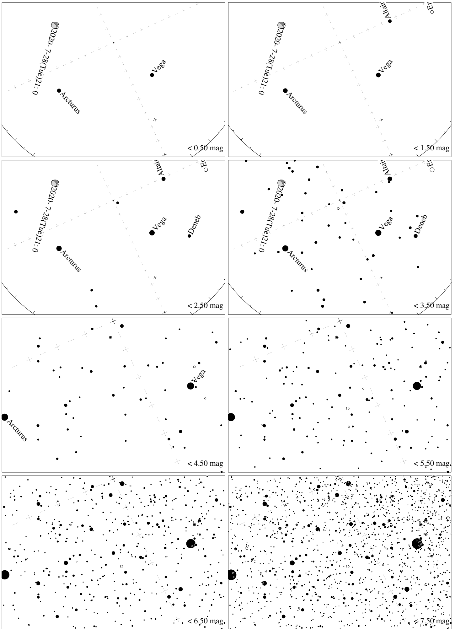
Maps for Globe at Night latitude 10^\circ , 2020-07-28, 21 h local time (Sun at -36^\circ ), transparent air. Lines from N(E,S,W) to zenith shown (crosses each 10^\circ ). Centered on \zeta Herculis, which is 25^\circ to the left from N, at 66^\circ height. Detailed maps 50^\circ vertically, the first four maps 100^\circ . Jan Hollan, CzechGlobe
