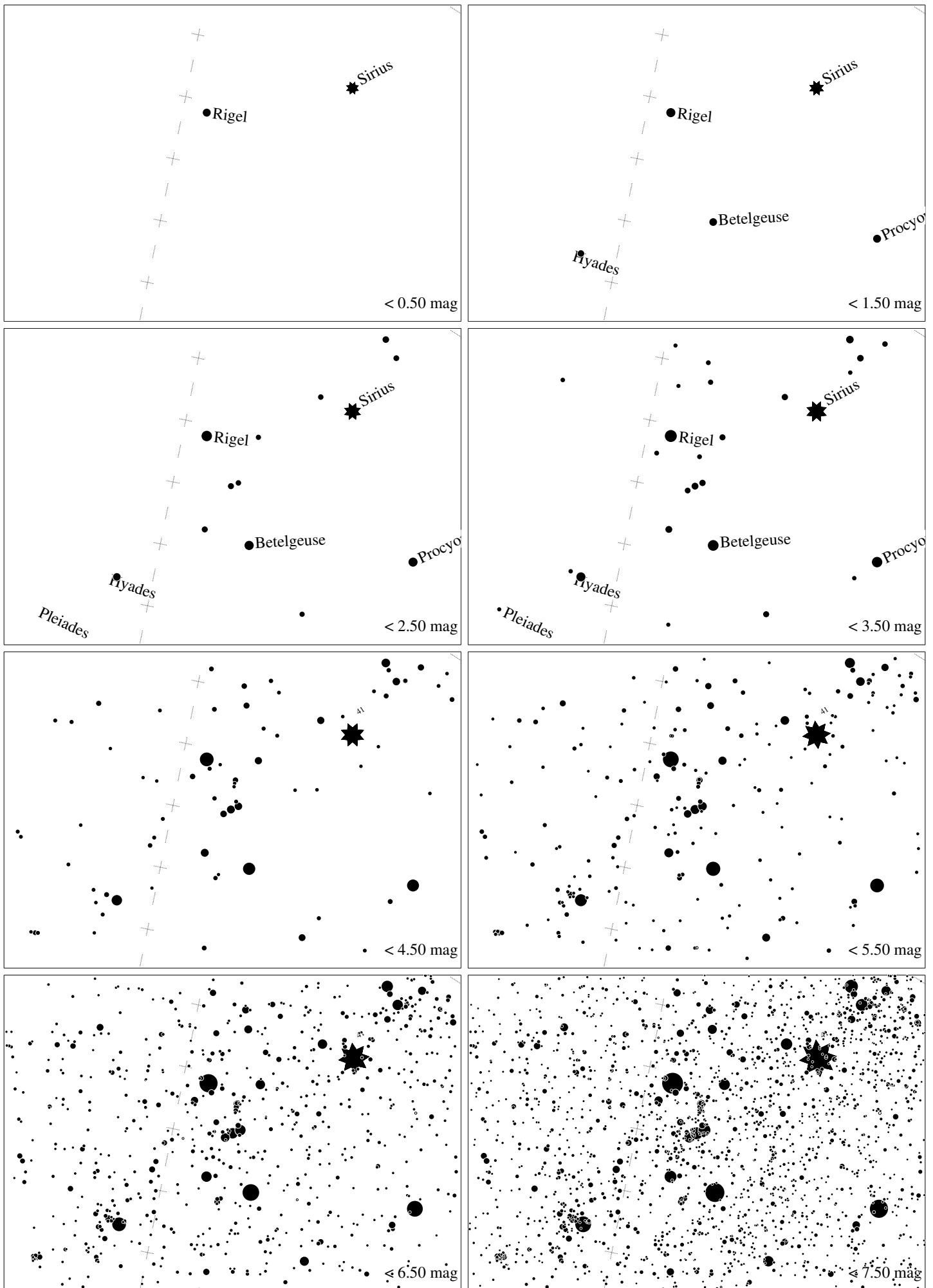
Maps for Globe at Night at latitude -40^\circ , 2020-01-20, 21 h local time (Sun at -15^\circ ), transparent air. Lines from N(E,S,W) to zenith shown (crosses each 10^\circ ). Orion 's belt is 15^\circ to the right from N, at 50^\circ height. Star clusters M 41 and M35 marked when appropriate. Map vertical size is 50^\circ . Jan Hollan maps, CzechGlobe
