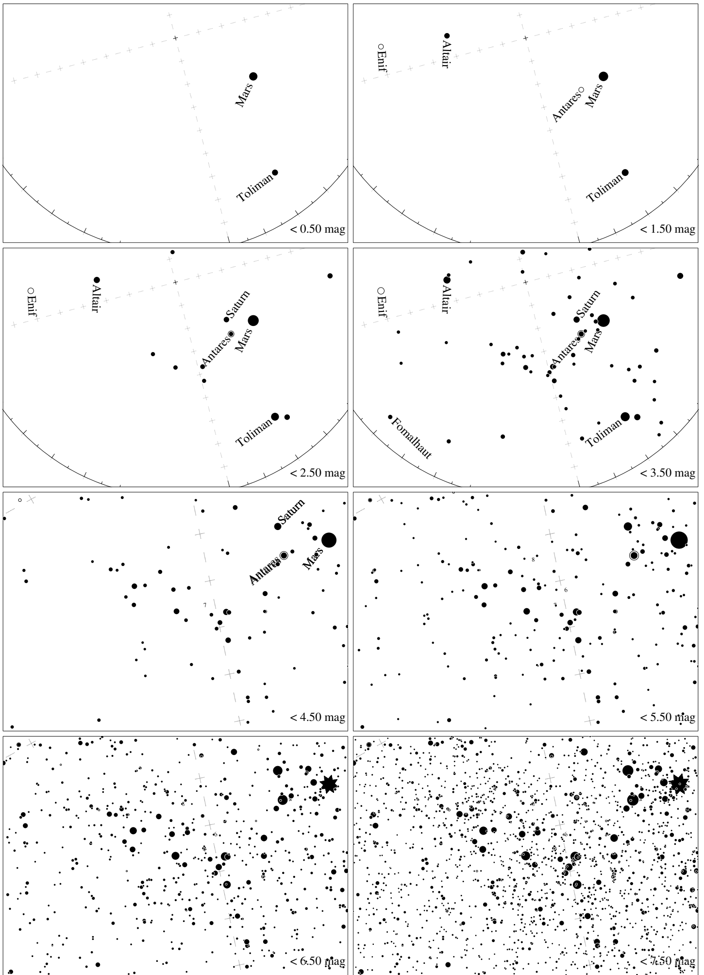
Maps for Globe at Night latitude 0^\circ , 2016-08-01, 21 h local time (Sun at -41^\circ ), transparent air. Lines from N(E,S,W) to zenith shown (crosses each 10^\circ ). Centered on Kaus Australis ( \epsilon Sagittarii), which is 15^\circ to the left from S, at 54^\circ height. Detailed maps 50^\circ vertically, the first four maps 100^\circ . Jan Hollan, CzechGlobe
