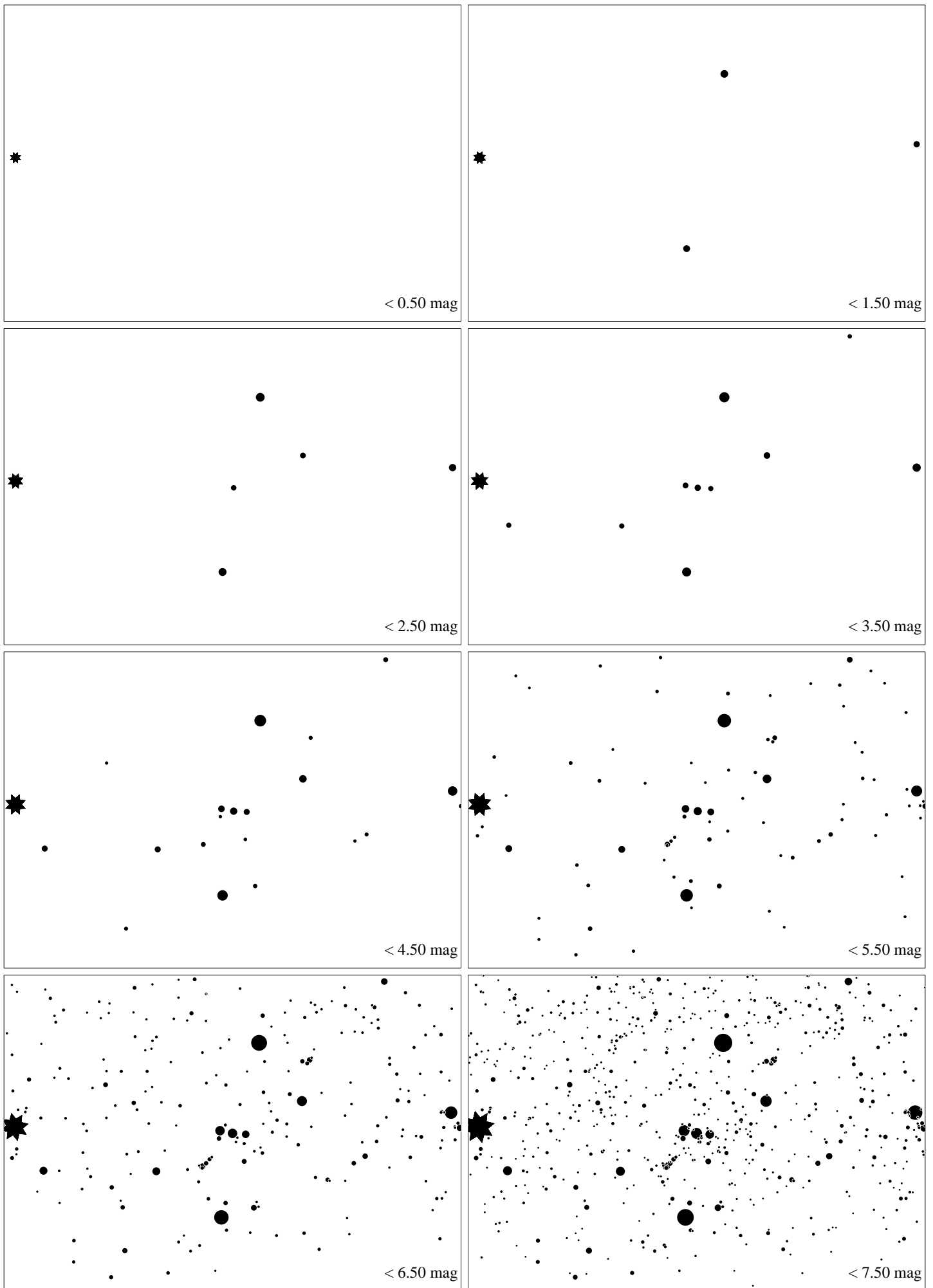
Maps for GLOBE at Night at latitude 40^\circ , March 30, 21 h local time (Mar 7, 22.5 h; Mar 23, 21.5 h, Apr 6, 20.5 h). Orion's belt is 68^\circ to the right from the south, at 23^\circ height. The brightest fixed star, Sirius, is at left. Jan Hollan, Ecological Institute Veronica and http://www.astro.cz/darksky
