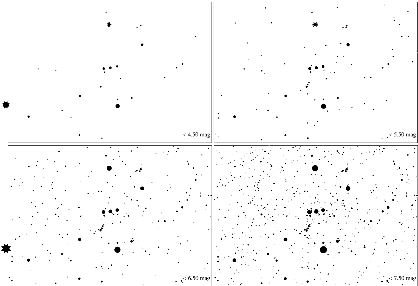
Maps for Globe at Night, lat. 49^\circ , Mar. 22, 20 h (end of astron. twilight), very clear air. Orion's belt is 30^\circ above SW. The brightest star, Sirius is just left from the plotted area. For more polluted skies, the numbers of visible stars would be 11 for a 3 mag limit, 5 for 2 mag , 2 for a 1 mag limit.
