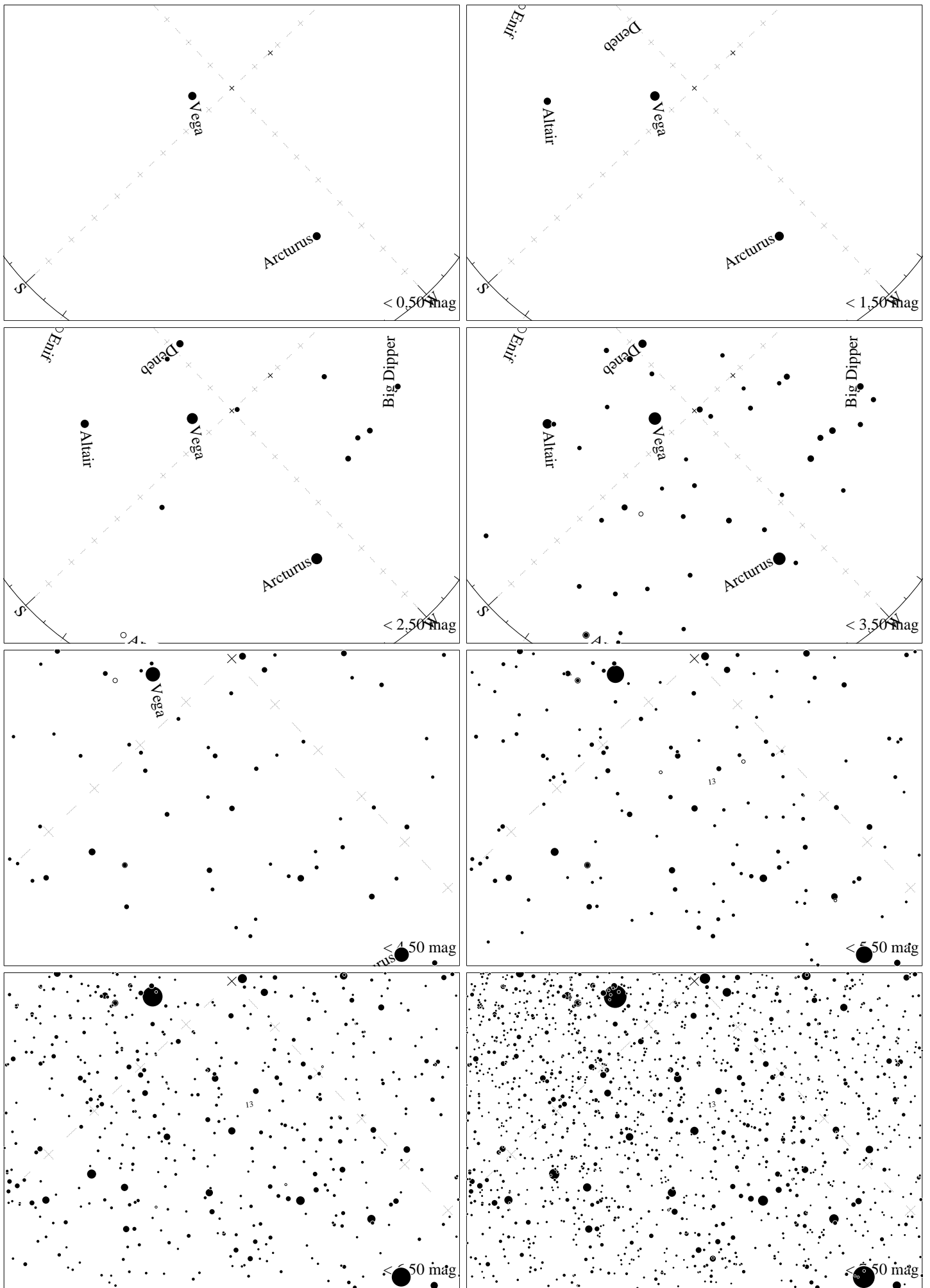
Maps for Globe at Night latitude 50^\circ , 2023-07-07, 23 h local time (Sun at -16^\circ ), transparent air. Lines from N(E,S,W) to zenith shown (crosses each 10^\circ ). Centered on \zeta Herculis, which is 47^\circ to the right from S, at 66^\circ height. Detailed maps 50^\circ vertically, the first four maps 100^\circ . Jan Hollan, CzechGlobe
