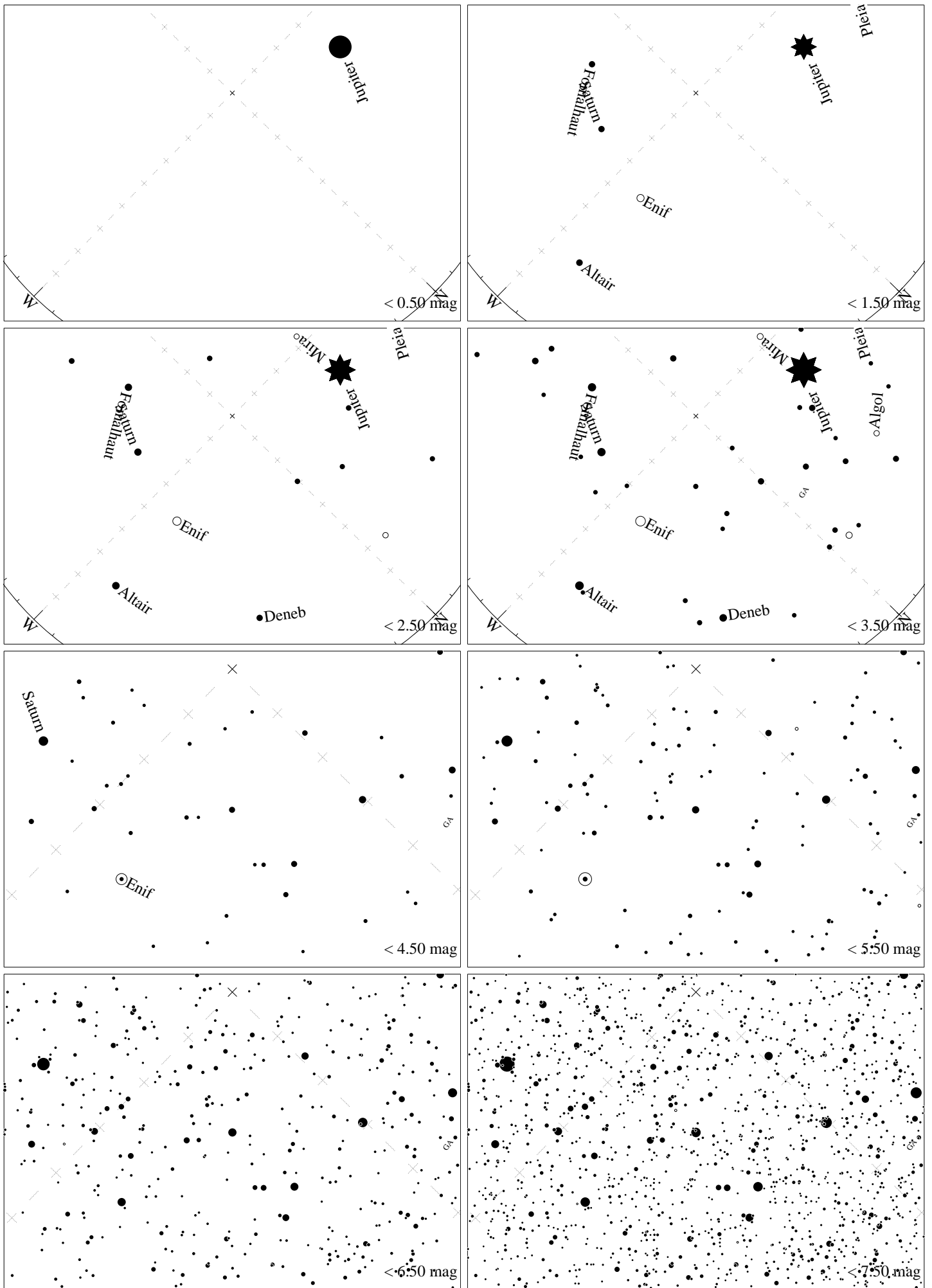
Maps for Globe at Night latitude 0^\circ , 2023-11-08, 21 h local time (Sun at -46^\circ ), transparent air. Lines from N(E,S,W) to zenith shown (crosses each 10^\circ ). The map is centered on Markab ( \alpha Pegasi), which is 46^\circ to the left from N, at 68^\circ height. Detailed maps 50^\circ vertically, the first four maps 100^\circ . Jan Hollan, CzechGlobe
