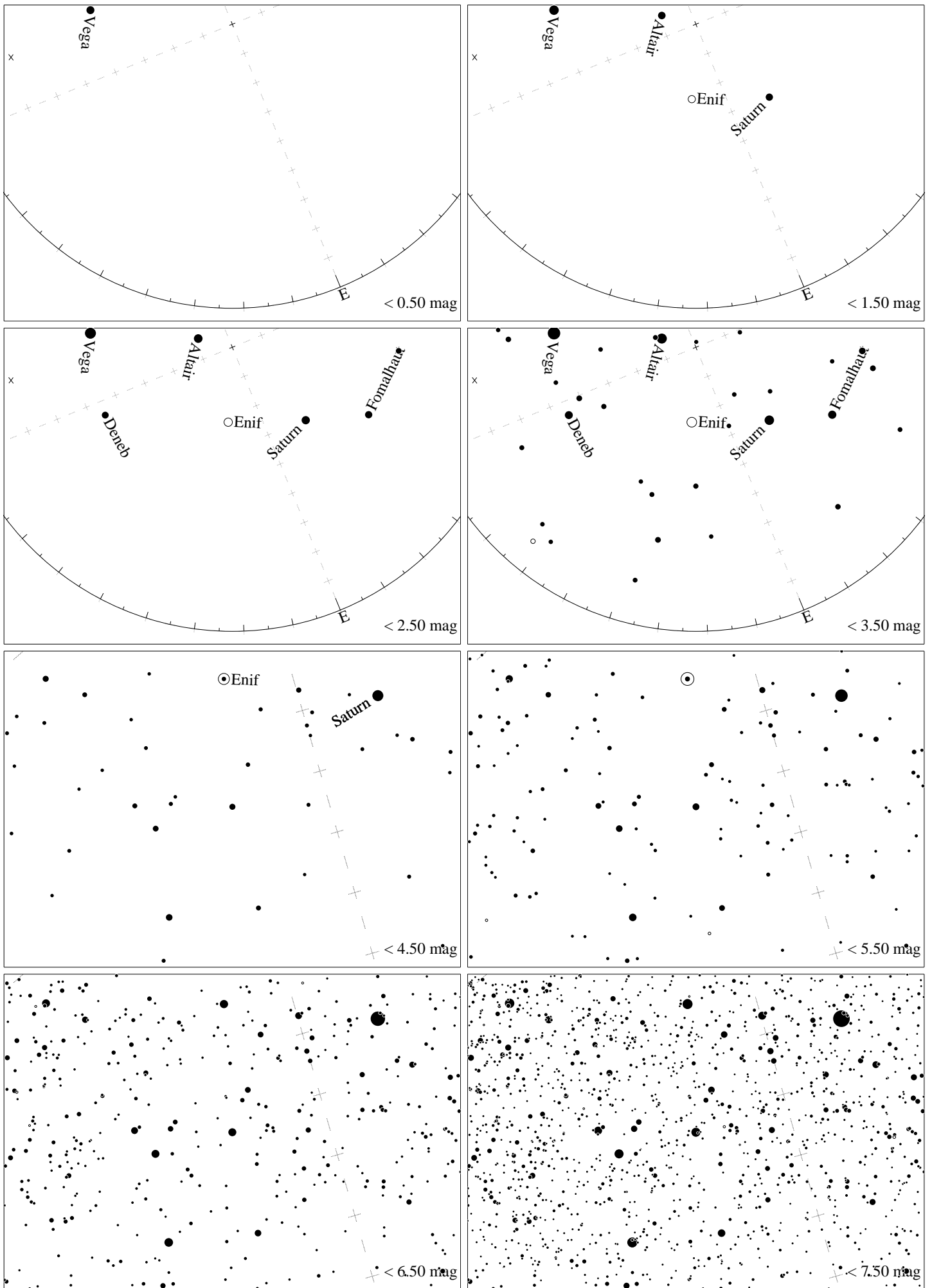
Maps for Globe at Night latitude 0°, 2023-09-10, 21 h local time (Sun at -46^\circ ), transparent air. Lines from N(E,S,W) to zenith shown (crosses each 10^\circ ). The map is centered on Markab ( \alpha Pegasi), which is 68^\circ to the right from N, at 46^\circ height. Detailed maps 50^\circ vertically, the first four maps 100^\circ . Jan Hollan, CzechGlobe
