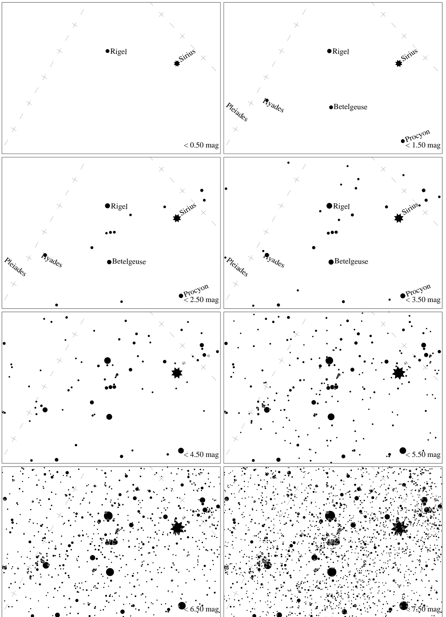
Maps for Globe at Night at latitude -30^\circ , 2021-01-09, 21 h local time (Sun at -21^\circ ), transparent air. Lines from N(E,S,W) to zenith shown (crosses each 10^\circ ). Orion's belt is 37^\circ to the right from N, at 56^\circ height. Star clusters M 41 and M35 marked when appropriate. Map vertical size is 50^\circ . Jan Hollan maps, CzechGlobe
