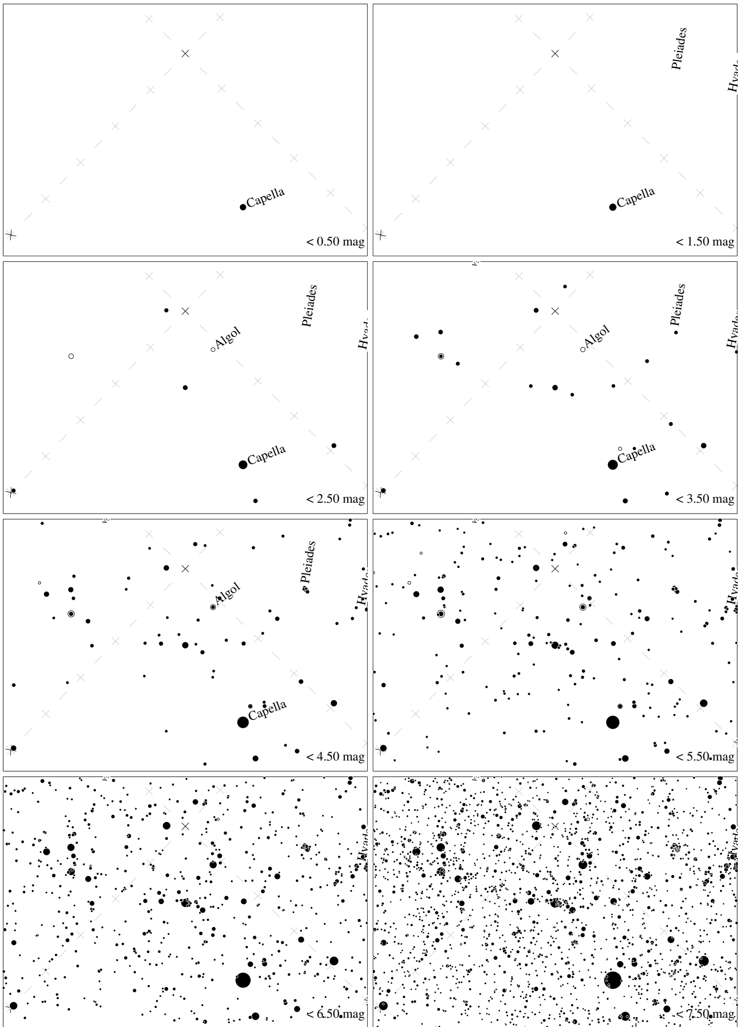
Maps for Globe at Night latitude 40°, 2020-12-10, 21 h local time (Sun at -50^\circ ), transparent air. Lines from N(E,S,W) to zenith shown (crosses each 10°). Centered at Mirfak ( \alpha Persei), 44° to the right from N, at 75° height. The brightest star is Capella. Map vertical size 50°. Jan Hollan, CzechGlobe
