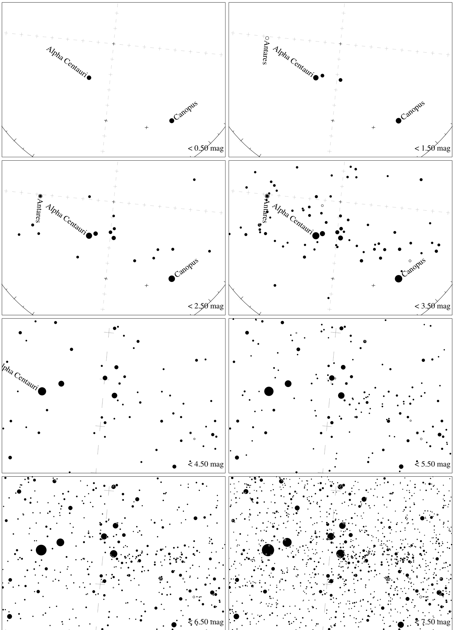
Maps for Globe at Night latitude -40^\circ , 2020-05-18, 21 h local time (Sun at -47^\circ ), transparent air. Central star Acrux (the brightest one in the Cross) is 6^\circ left from the south, at 67^\circ height. Detailed maps 33^\circ vertically, the first four maps 100^\circ . Jan Hollan, CzechGlobe
