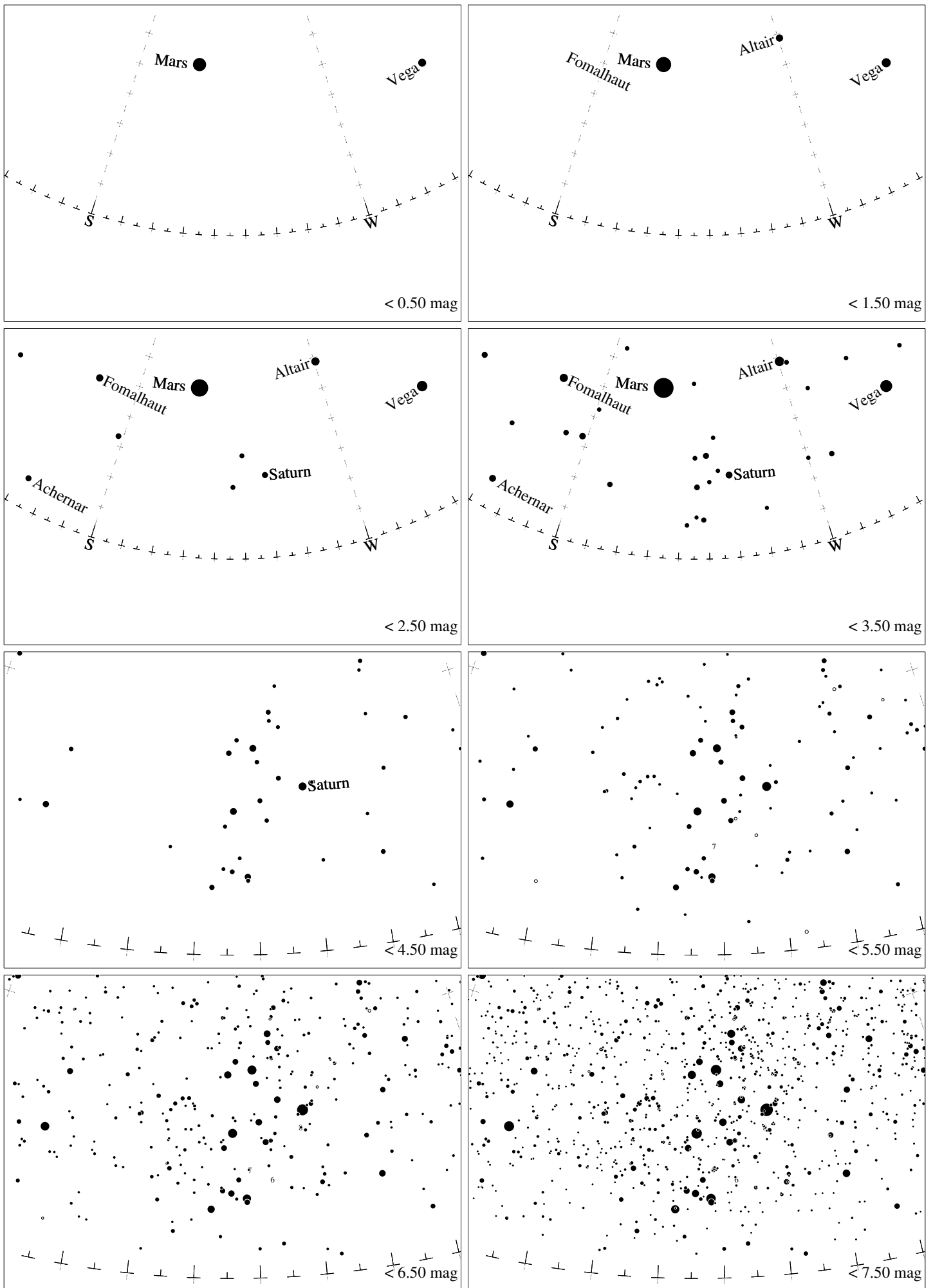
Maps for Globe at Night latitude 10°, 2018-10-05, 21 h local time (Sun at -48^\circ ), transparent air. Lines from N(E,S,W) to zenith shown (crosses each 10°). Centered on Kaus Australis ( \epsilon Sagittarii), which is 46^\circ to the right from S, at 23^\circ height. Detailed maps 50^\circ vertically, the first four maps 100^\circ . Jan Hollan, CzechGlobe
