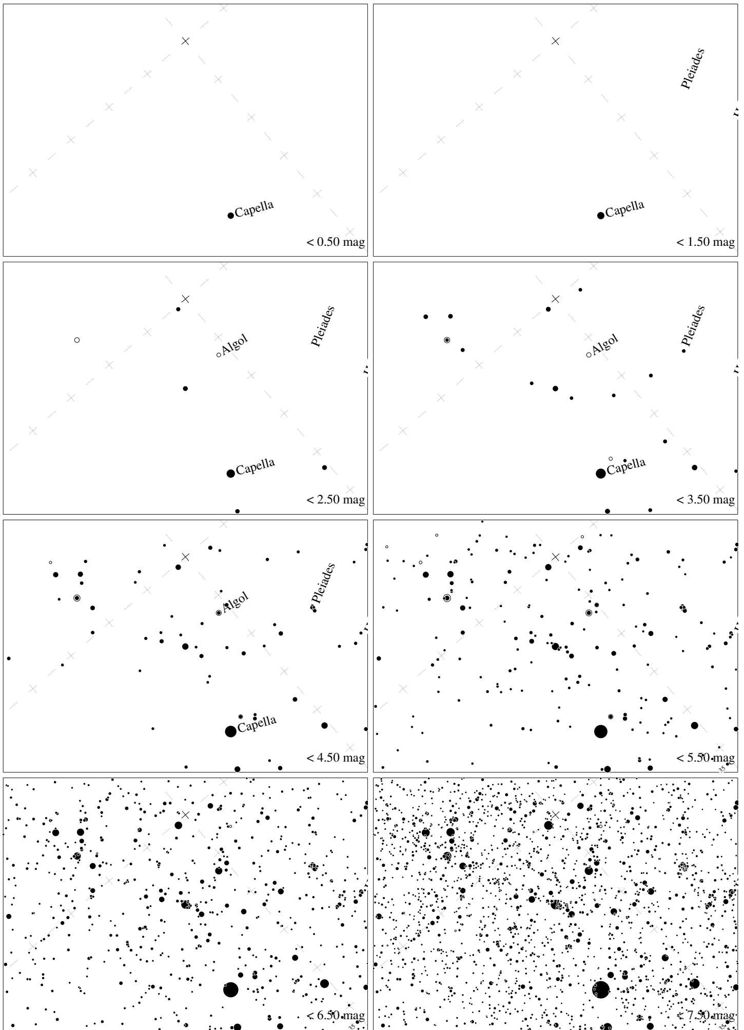
Maps for Globe at Night latitude 40°, 2015-12-06, 21 h local time (Sun at -50^\circ ), transparent air. Lines from N(E,S,W) to zenith shown (crosses each 10^\circ ). Centered at Mirfak ( \alpha Persei), 49^\circ to the right from N, at 72^\circ height. The brightest star is Capella. Map vertical size 50^\circ . Jan Hollan, CzechGlobe
