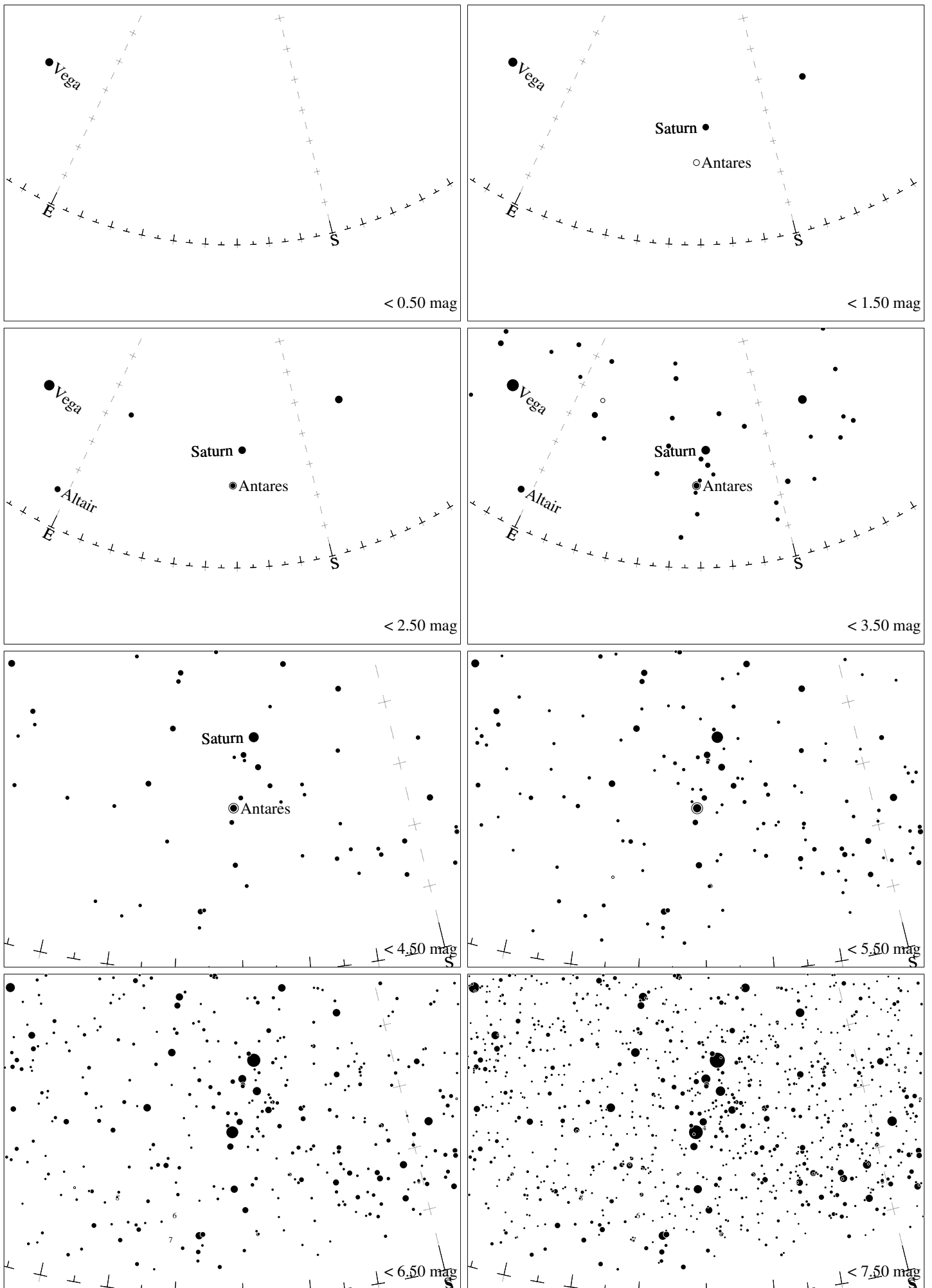
Maps for Globe at Night latitude 30°, 2015-06-12, 21 h local time (Sun at -22°), transparent air. Lines from N(E,S,W) to zenith shown (crosses each 10°). Centered on Antares ( \alpha Scorpii), which is 32° to the left from S, at 26° height. Detailed maps 50° vertically, the first four maps 100°. Jan Hollan, CzechGlobe
