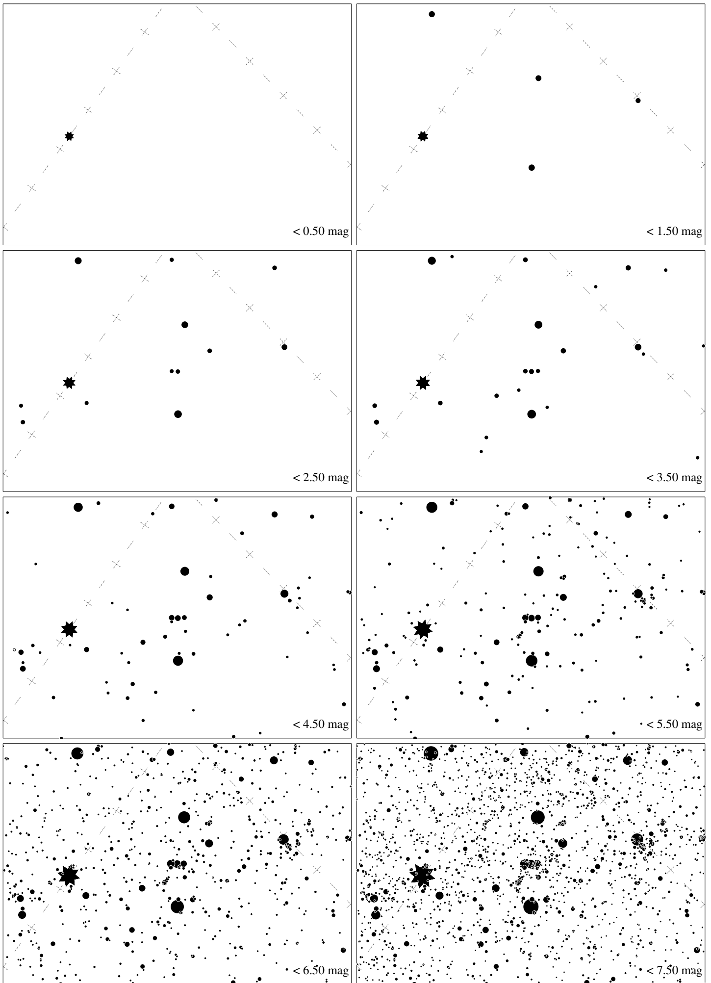
Maps for Globe at Night at latitude 20^\circ , February 16, 21 h local time (Sun at -43^\circ ), assuming rather turbid air. Lines from N(E,S,W) to zenith shown (crosses each 10^\circ ). Orion's belt is 40^\circ to the right from S, at 63^\circ height. The brightest star is Sirius. Map vertical size is 50^\circ . Jan Hollan, CzechGlobe
