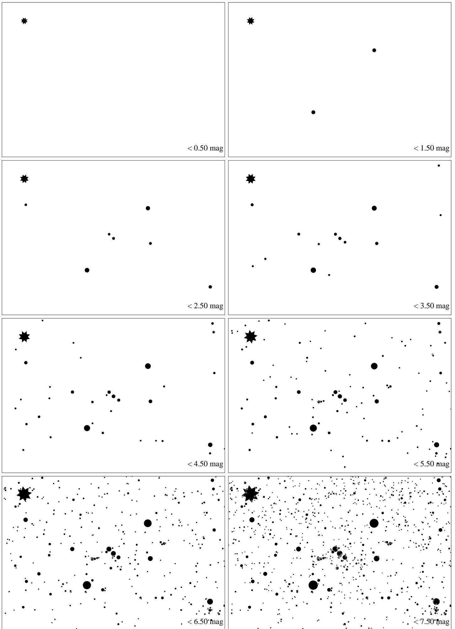
Maps for GLOBE at Night at latitude 10^\circ , March 30, 21 h local time (Mar 7, 22.5 h; Mar 23, 21.5 h, Apr 6, 20.5 h). Orion's belt is 83^\circ to the right from the south, at 31^\circ height. The brightest fixed star, Sirius, is at upper left. Jan Hollan, Ecological Institute Veronica and http://www.astro.cz/darksky
