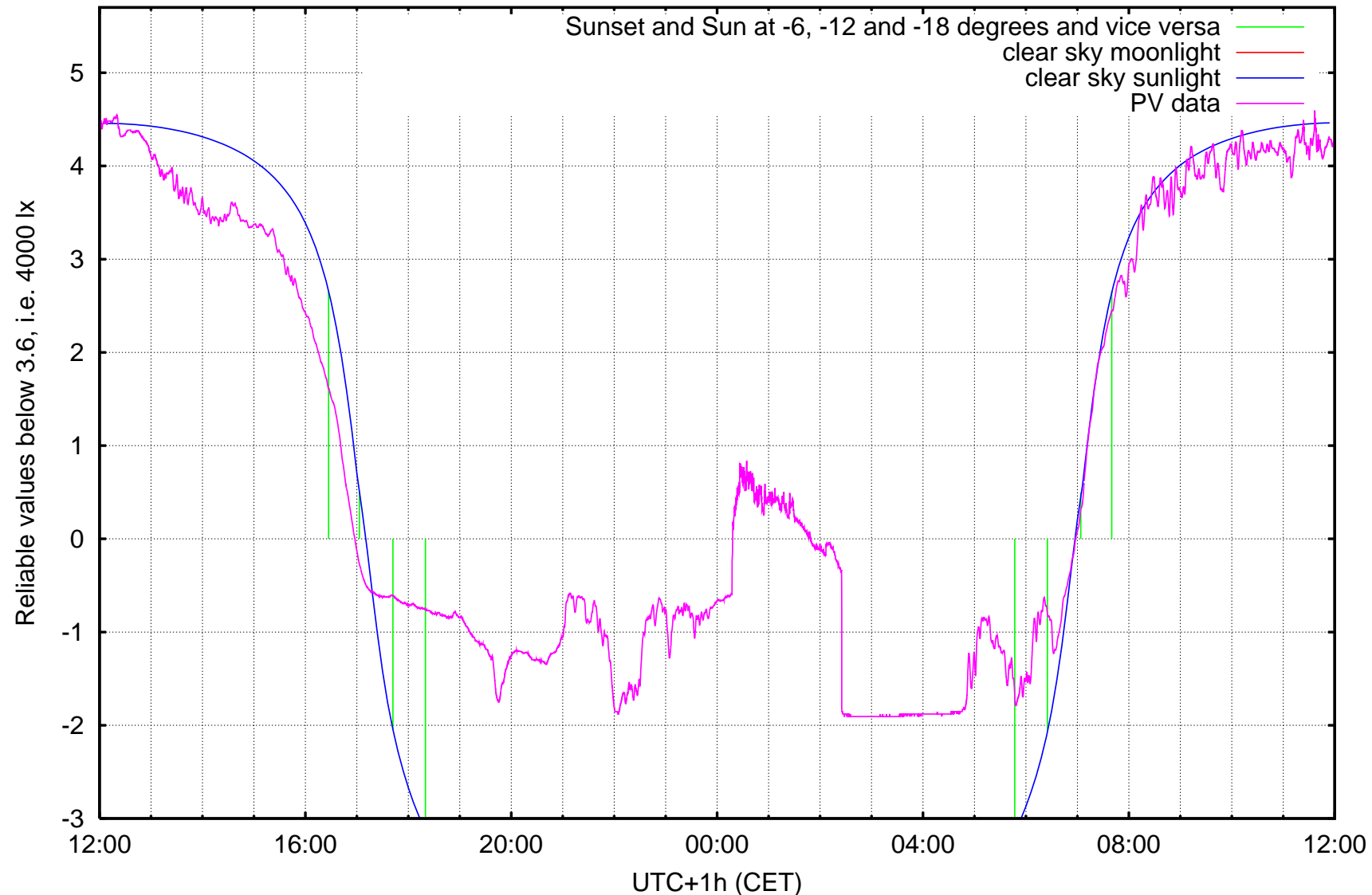
log10 ( illuminance / 1 lx ) Kravi hora, Brno, ending at Friday 2007-01-19 noon
