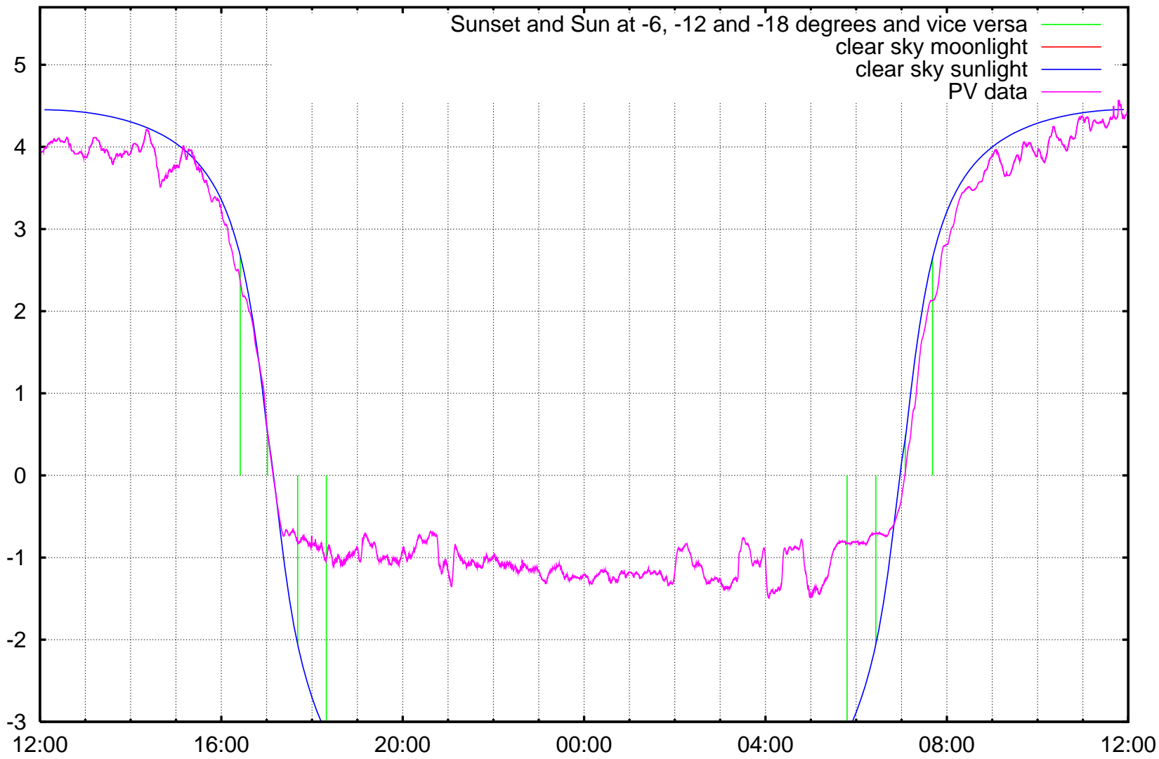
log10 ( illuminance / 1 lx ) Kravi hora, Brno, ending at Thursday 2007-01-18 noon
