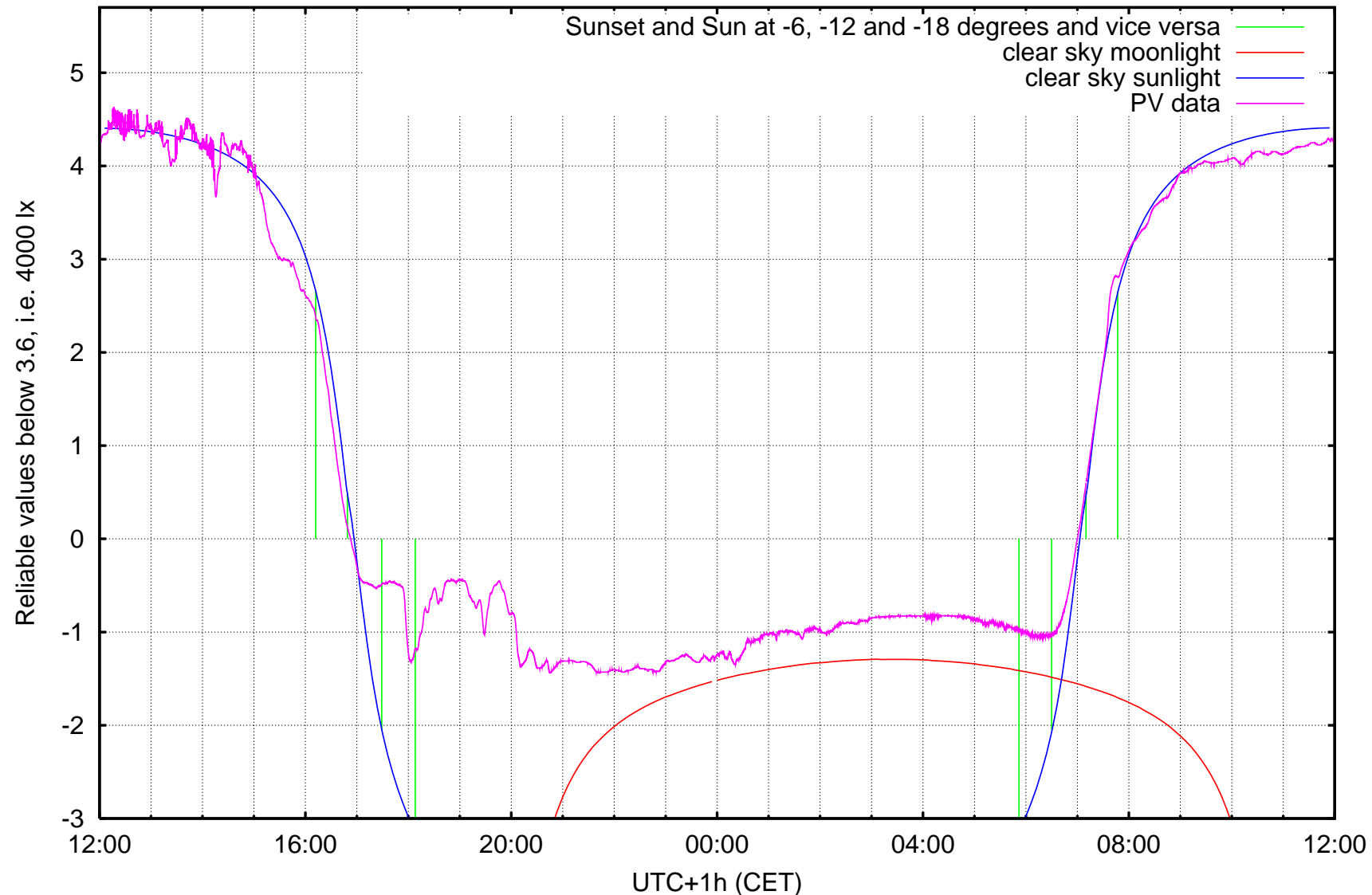
log10 ( illuminance / 1 lx ) Kravi hora, Brno, ending at Monday 2007-01-08 noon
