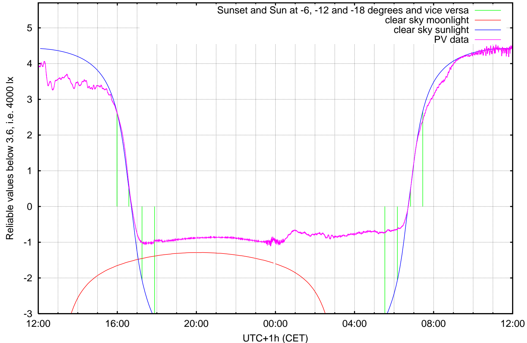
log10 ( illuminance / 1 lx ) Kravi hora, Brno, ending at Friday 2006-12-01 noon
