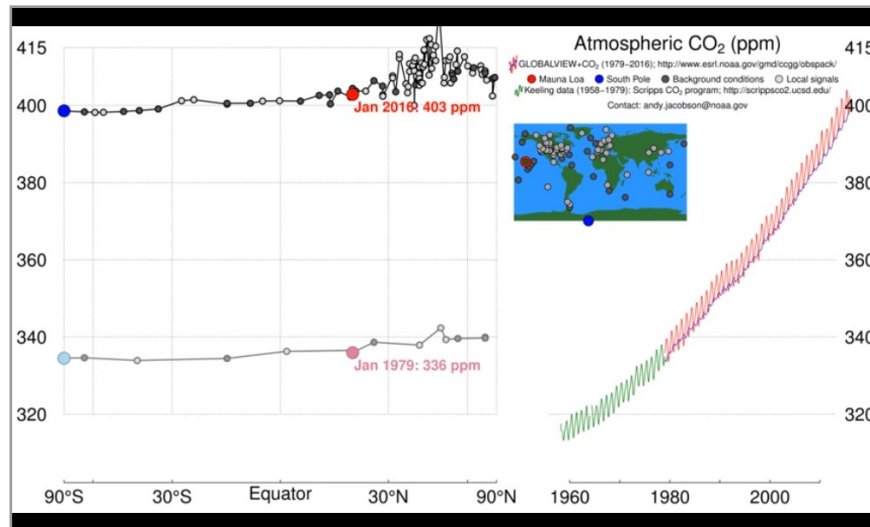
Atmospheric CO 2 at Mauna Loa Observatory
