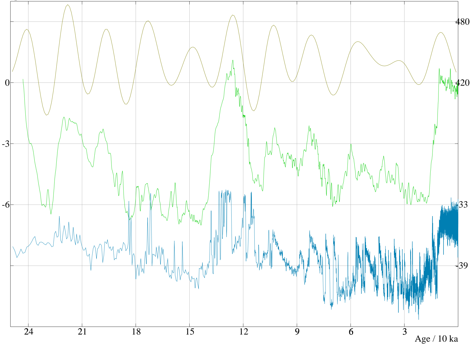
temperature - that in 1990 / K (middle, Vostok data) top: mid-July mean insolation of 65N latitude / W.m-2, bottom: GRIP O18 data
