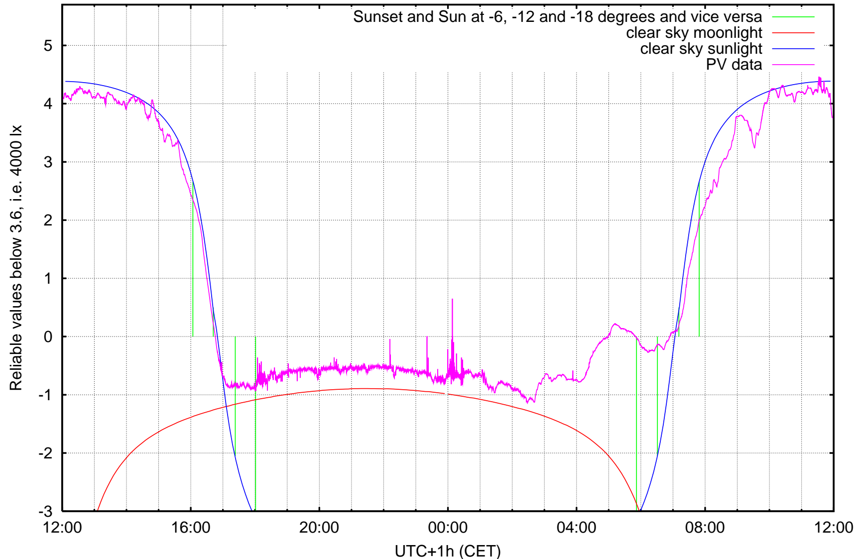
log10 ( illuminance / 1 lx ) Kravi hora, Brno, ending at Monday 2007-01-01 noon
