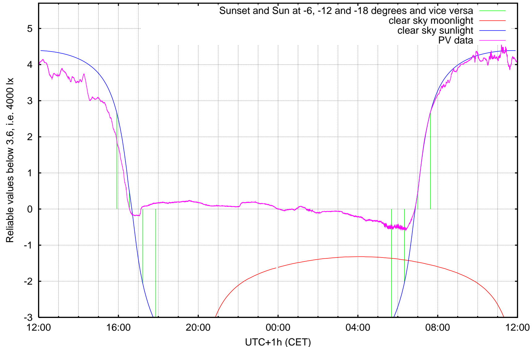
log 10 ( illuminance / 1 lx ) Kravi hora, Brno, ending at Sunday 2006-12-10 noon
