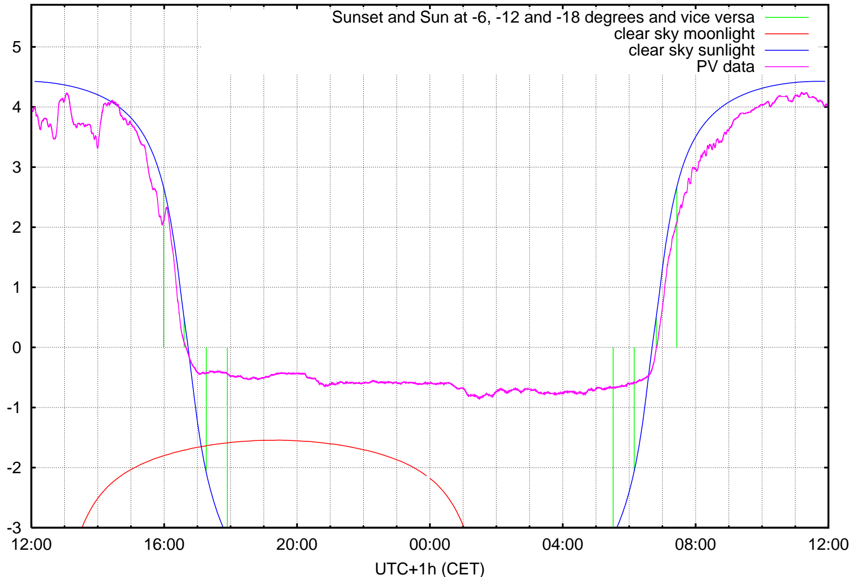
log10 ( illuminance / 1 lx ) Kravi hora, Brno, ending at Thursday 2006-11-30 noon
