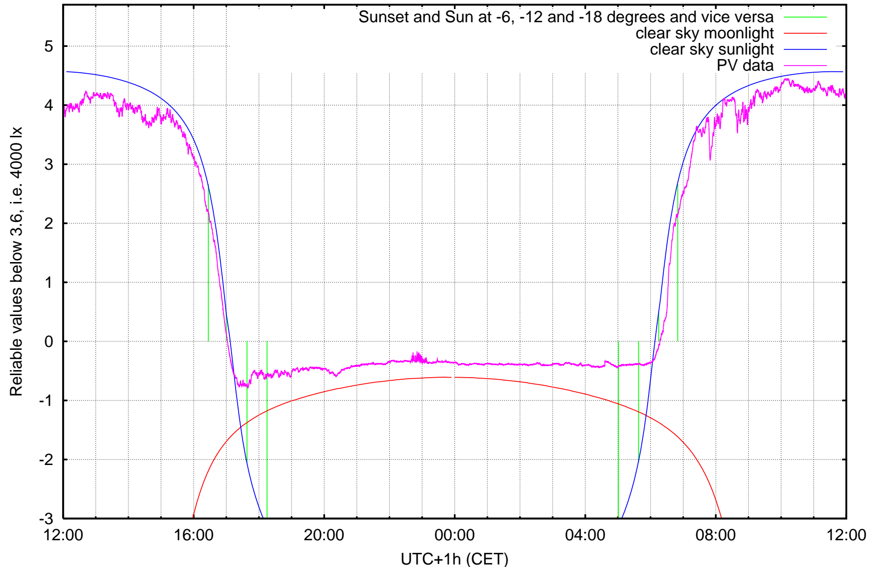
log10 ( illuminance / 1 lx ) Kravi hora, Brno, ending at Monday 2006-11-06 noon
