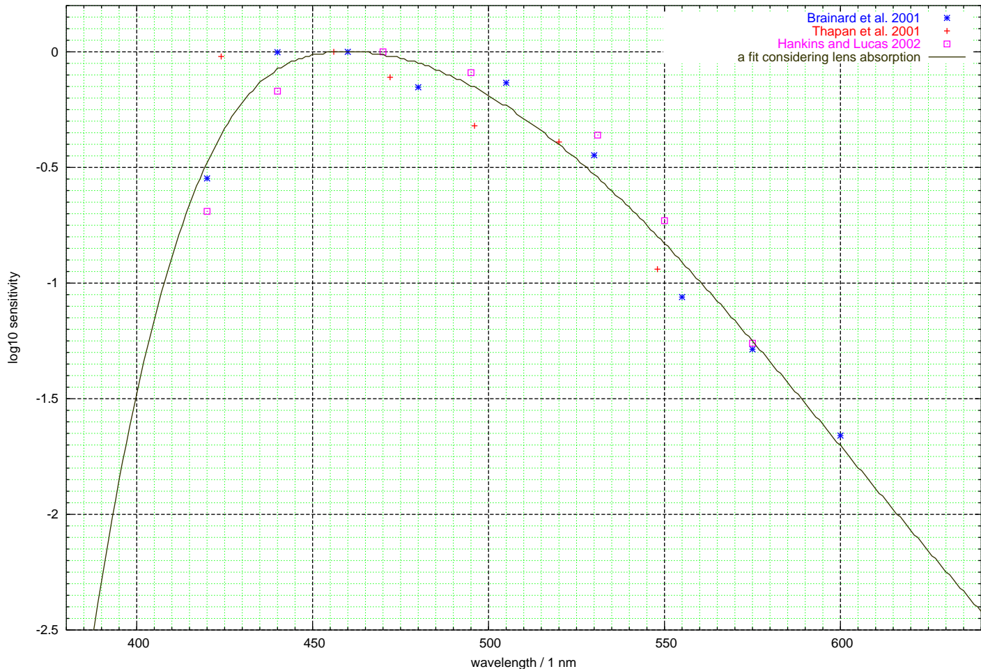
Action spectrum of melanin suppression by light
