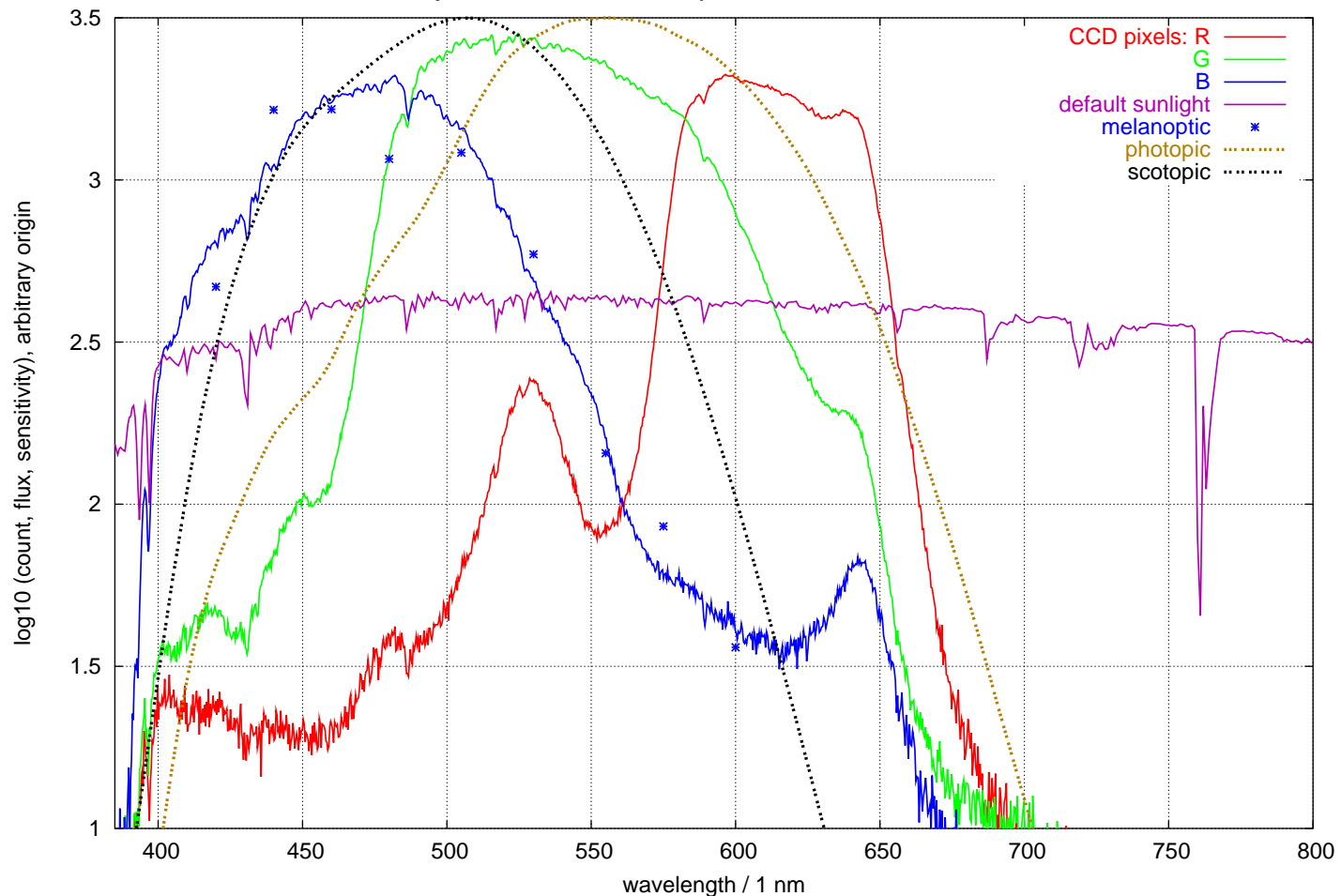
Fuji S5000 raw solar spectrum at 'airmass=1.5'
