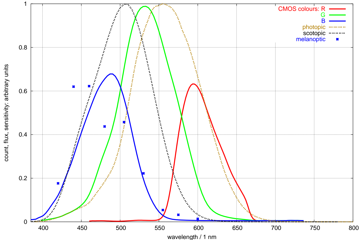
Canon EOS D60 spectral sensitivity (preliminary)
