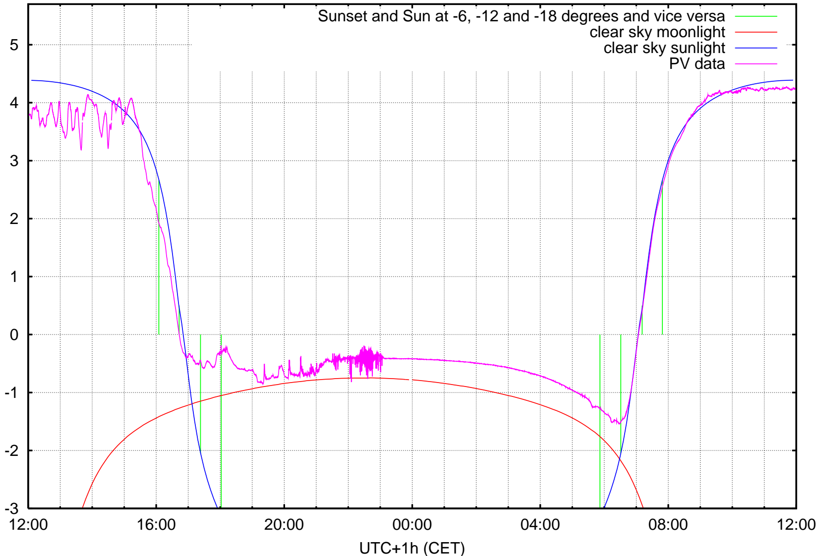
log10 ( illuminance / 1 lx ) Kravi hora, Brno, ending at Tuesday 2007-01-02 noon
