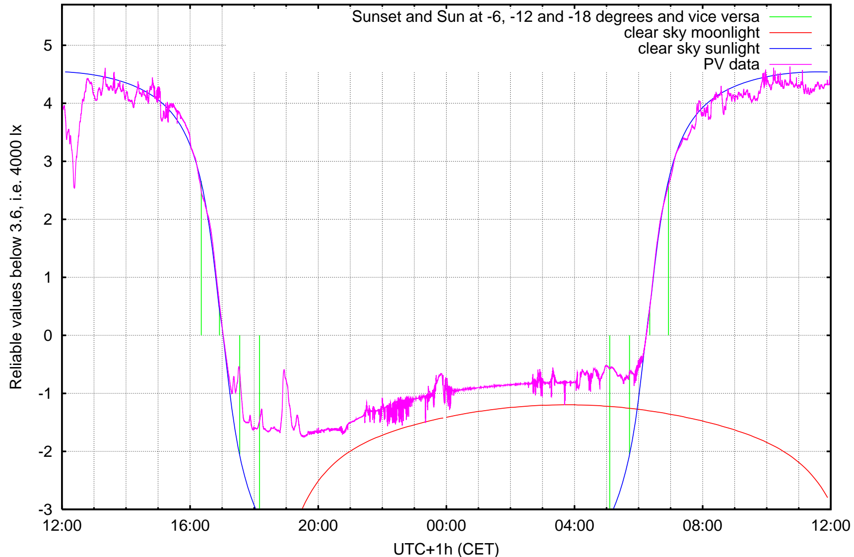
log10 ( illuminance / 1 lx ) Kravi hora, Brno, ending at Friday 2006-11-10 noon
