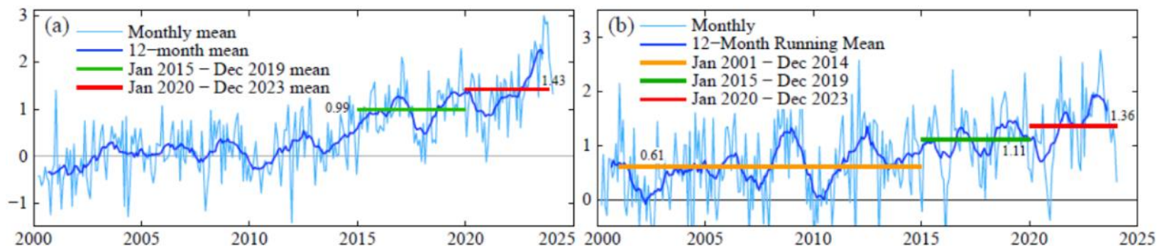
Fig. 7. (a) Global absorbed solar radiation (ASR) relative to the mean of the first 120 months of CERES data (W/m 2 ). 6 (b) Earth's energy imbalance (EEI) from CERES satellite data normalized to the 0.71 W/m 2 mean for July 2005 – June 2015 based on Argo and other data. 7 CERES data are available at http://ceres.larc.nasa.gov/order_data.php
