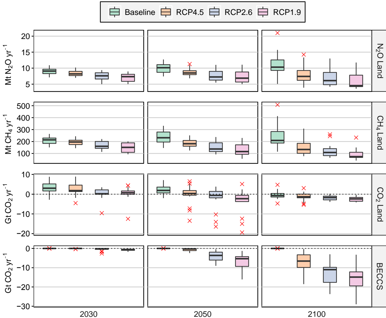
10 Figure 2.25 Land-based global GHG emissions and removals in 2030, 2050 and 2100 for Baseline, RCP4.5, 11 RCP2.6 and RCP1.9 based on the Shared Socioeconomic Pathways (SSP) (Popp et al. 2017; Rogelj et al. 12 2018; Riahi et al. 2017). Data is from an update of the IAMC Scenario Explorer developed for the SR15 13 (Huppmann et al. 2018; Rogelj et al. 2018). Boxplots (Tukey style) show median (horizontal line), 14 interquartile range (IQR box) and the range of values within 1.5 x IQR at either end of the box (vertical 15 lines) across 5 SSPs and across 5 IAMs. Outliers (red crosses) are values greater than 1.5 x IQR at either 16 end of the box. The categories CO 2 Land, CH 4 Land and N 2 O Land include GHG emissions from land-use 17 change and agricultural land use (including emissions related to bioenergy production). In addition, the 18 category CO 2 Land includes negative emissions due to afforestation. BECCS reflects the CO 2 emissions 19 captured from bioenergy use and stored in geological deposits.
