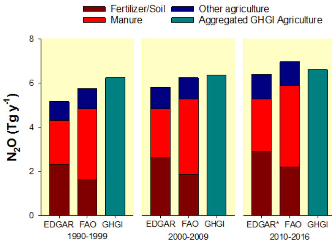
24 25 Figure 2.11 Average agricultural N 2 O emissions estimates from 1990. Sub-sectorial agricultural emissions 26 are based on the Emissions Database for Global Atmospheric Research (EDGAR v4.3.2; Janssens- 27 Maenhout et al. 2017a); FAOSTAT (Tubiello et al. 2013); and National GHGI data (Grassi et al. 2018). 28 GHGI data are aggregate values for the sector.
