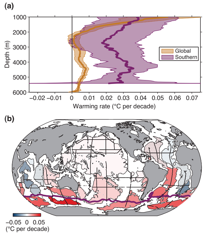
Figure 3.3 | (a) Areal mean warming rates ( ^{\circ}\text{C} per decade) versus depth (thick lines) with 5 to 95% confidence limits (shading), both global (orange) and south of the Sub-Antarctic Front (purple), centred on 1992–2005. (b) Mean warming rates ( ^{\circ}\text{C} per decade) below 4000 m (colour bar) estimated for deep ocean basins (thin black outlines), centred on 1992–2005. Stippled basin warming rates are not significantly different from zero at 95% confidence. The positions of the Sub-Antarctic Front (purple line) and the repeat oceanographic transects from which these warming rates are estimated (thick black lines) also shown. (Data from Purkey and Johnson, 2010.)
