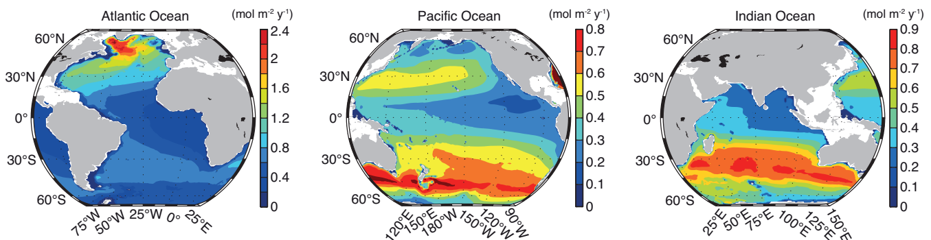
Figure 3.17 | Maps of storage rate distribution of anthropogenic carbon ( \text{mol m}^{-2} \text{ yr}^{-1} ) for the three ocean basins (left to right: Atlantic, Pacific and Indian Ocean) averaged over 1980–2005 estimated by the Green's function approach (Khatiwala et al., 2009). Note that a different colour scale is used in each basin.
