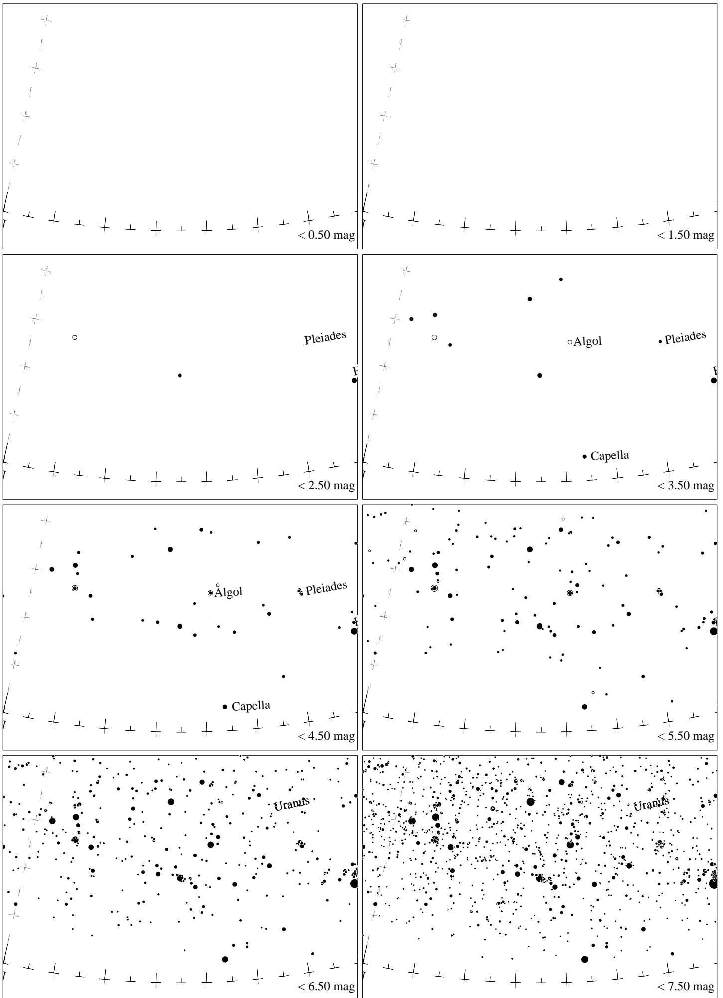
Maps for Globe at Night latitude 0°, 2023-11-01, 21 h local time (Sun at -47^\circ ), transparent air. Lines from N(E,S,W) to zenith shown (crosses each 10^\circ ). Centered at Mirfak ( \alpha Persei), 35^\circ to the right from N, at 21^\circ height. The brightest star is Capella. Map vertical size 50^\circ . Jan Hollan, CzechGlobe
