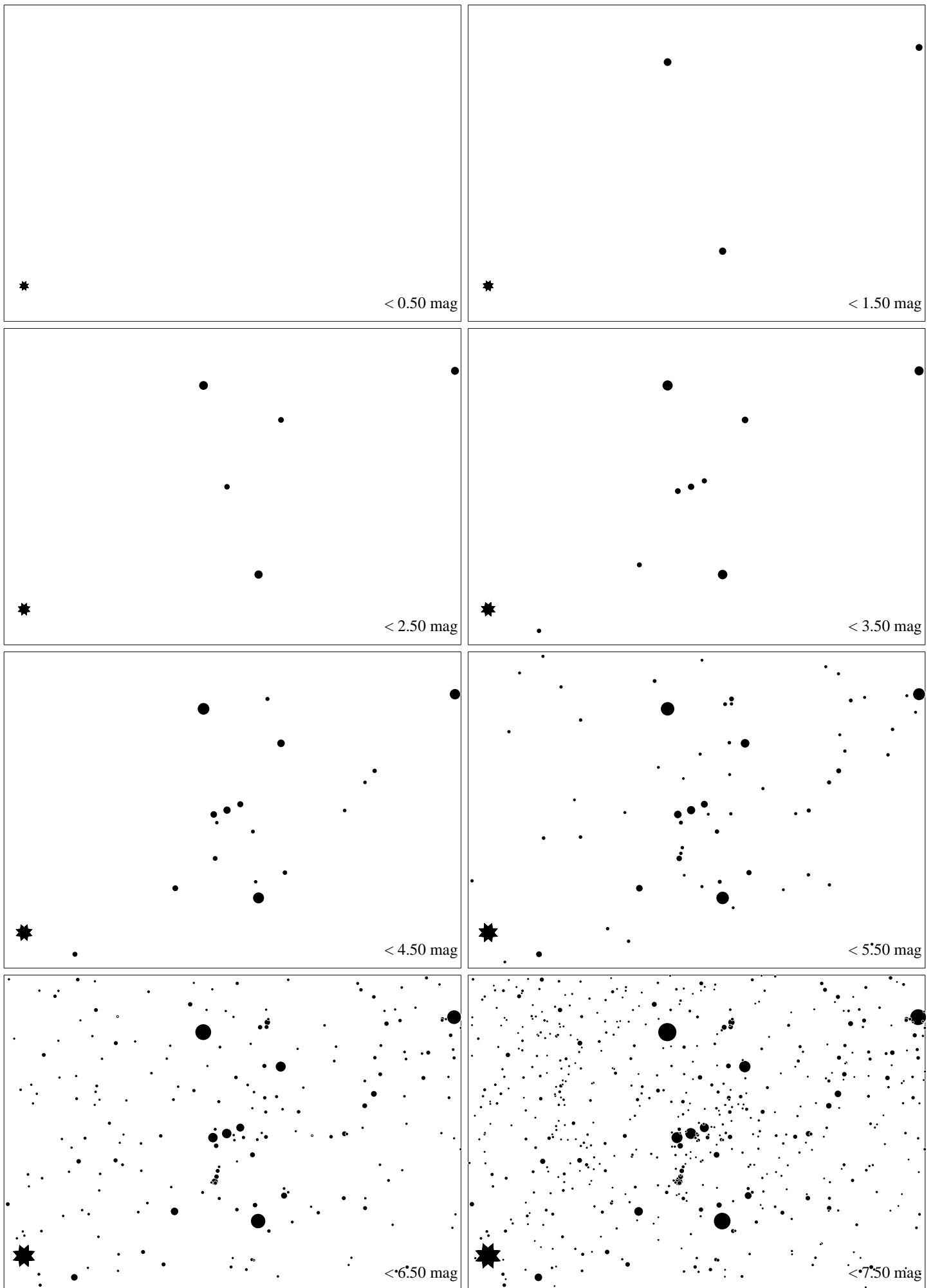
Maps for Globe at Night at latitude 60^\circ N, March 10, 20:30 local time (after astronomic twilight), assuming rather transparent air. Orion's belt is 35^\circ to the right from the south, 24^\circ high. The brightest fixed star, Sirius, is at left. J.H., N. Copernicus Observatory and Planetarium in Brno and http://www.astro.cz/darksky
