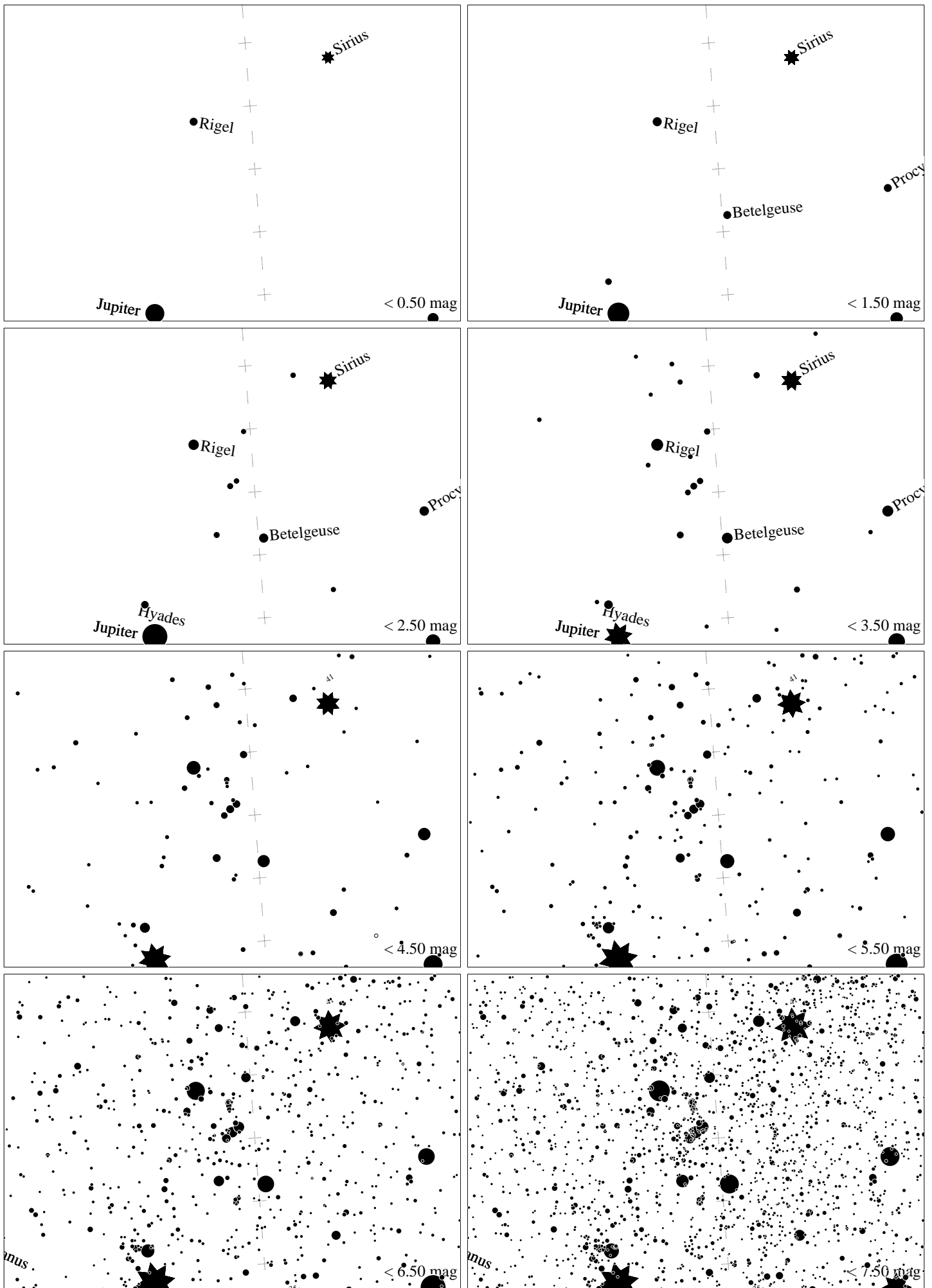
Maps for Globe at Night at latitude -40^\circ , 2025-01-25, 21:30 local time (Sun at -20^\circ ), transparent air. Lines from N(E,S,W) to zenith shown (crosses each 10^\circ ). Orion 's belt is 6^\circ to the left from N, at 51^\circ height. Star clusters M 41 and M35 marked when appropriate. Map vertical size is 50^\circ . Jan Hollan maps, CzechGlobe
